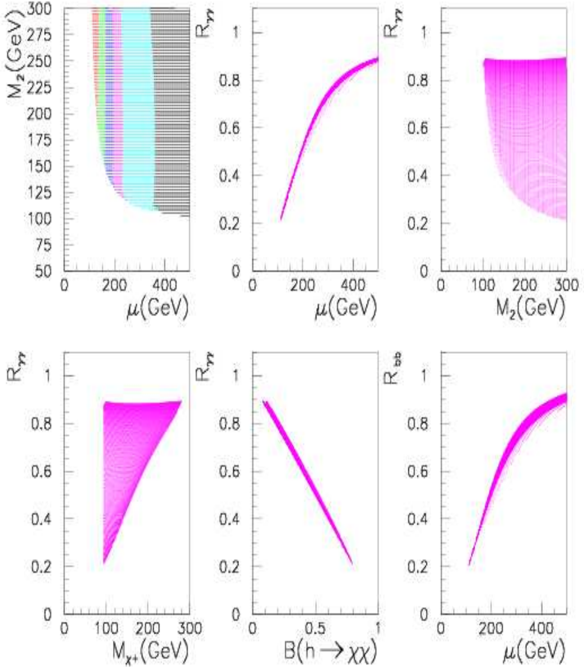
Figure 13: Effects of neutralinos from M_1 = M_2/10 with \tan\beta = 5 and A_t = 0 with heavy selectrons. In all the plots, scans are over M_2 = 50 - 300 \text{ GeV} , \mu = 100 - 500 \text{ GeV} . From left to right and top to bottom a) Density plot for R_{\gamma\gamma} in the allowed M_2 - \mu plane. The different shadings correspond to .3 < R_{\gamma\gamma} < .4 (left band) to .8 < R_{\gamma\gamma} < .9 (right band). b) Variation of R_{\gamma\gamma} with \mu c) with M_2 d) with the mass of the chargino M_{\chi_1^+} . e) Correlation between R_{\gamma\gamma} and the branching into LSP. f) Variation of R_{b\bar{b}} with \mu .
