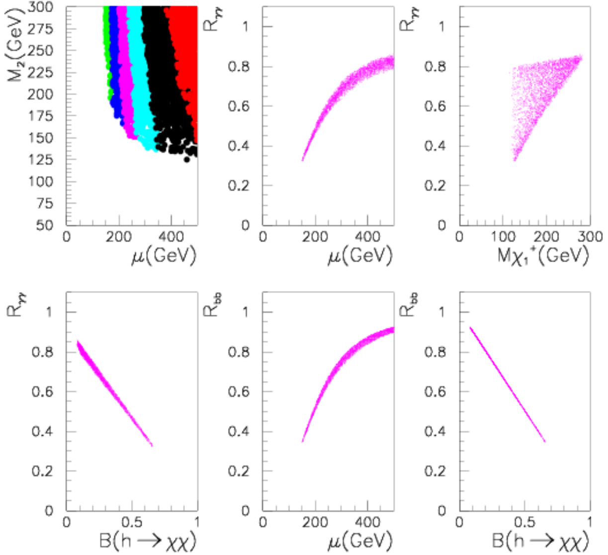
Figure 15: Effects of neutralinos from M_1 = M_2/10 with \tan \beta = 5 and A_t = 0 with light selectrons. In all plots the scans are over M_2 = 50 - 300 \text{ GeV} , \mu = 100 - 500 \text{ GeV} . From left to right and top to bottom a) Density plot for R_\gamma in the allowed M_2 - \mu plane. The different shadings correspond to .3 < R_\gamma < .4 (left band) to .8 < R_\gamma < .9 (right band). b) Variation of R_\gamma with \mu c) with the mass of the chargino M_{\chi_1^+} . d) Correlation between R_\gamma and the branching into LSP. e) Variation of R_{b\bar{b}} with \mu . f) R_{b\bar{b}} vs the branching of the Higgs into the LSP neutralino. .
