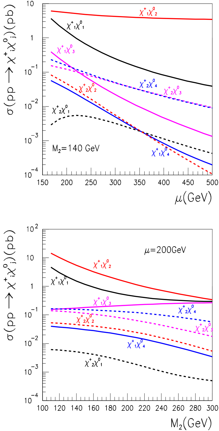
Figure 7: Associated Production of chargino and neutralino at the LHC at LO a) as a function of \mu for M_2 = 140 GeV. b) as a function of M_2 for \mu = 200 GeV. In the case of gaugino mass unification without degeneracy with the sneutrinos, the LEP limit means that for M_2 = 140 GeV, \mu > 176 GeV and for \mu = 200 GeV, M_2 > 130 GeV. In the case of degeneracy with the sneutrinos all points in the figure are valid .
