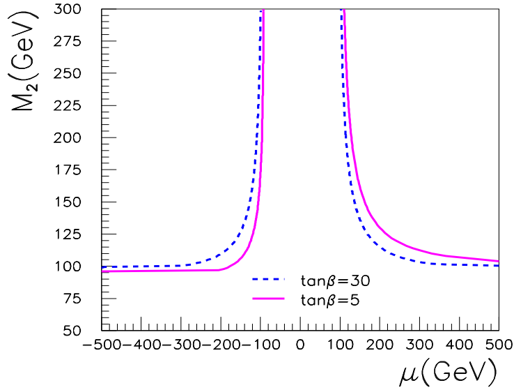
Figure 3: LEP2 excluded region (inside the branch) in the M_2 - \mu parameter space for \tan \beta = 5 and \tan \beta = 30 from m_{\chi_1^+} \geq 94.5 \text{ GeV} .
