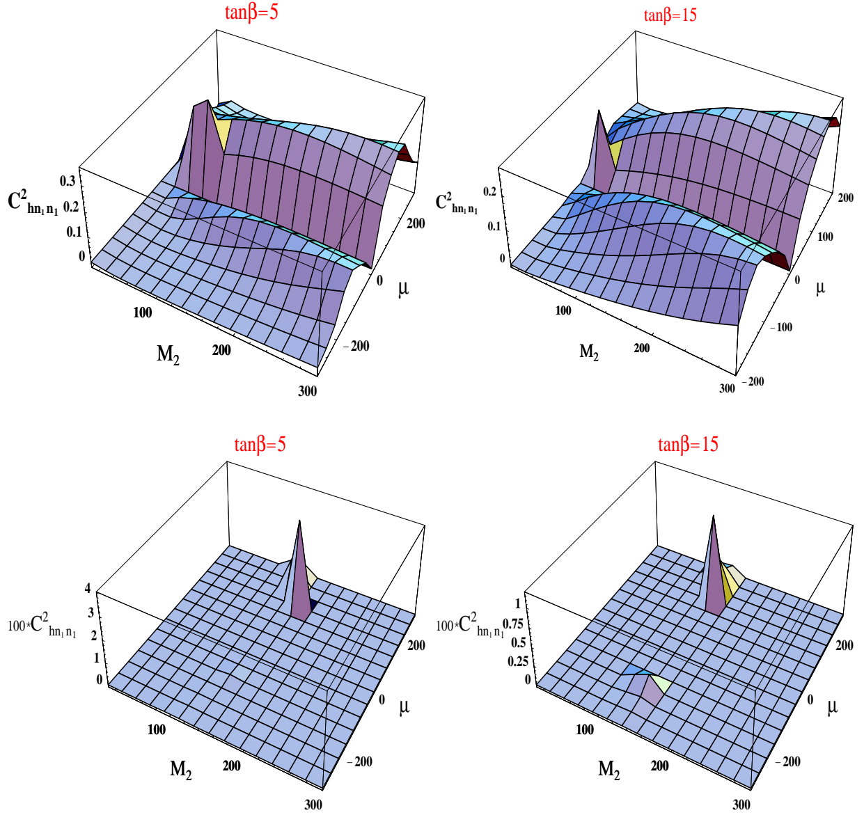
Figure 1: Strength of the lightest Higgs coupling to \tilde{\chi}_1^0 \tilde{\chi}_1^0 for \tan\beta = 5 and \tan\beta = 15 . In the second set (bottom) of figures we have imposed m_{\tilde{\chi}_1^\pm} > 94.5\text{GeV} (the current limit on the lightest chargino) and m_{\tilde{\chi}_1^0} < 65\text{GeV} (this corresponds to the threshold for the lightest Higgs with a maximum mass of about 130\text{GeV} to decay into the LSP neutralino). Here C_{hn_1 n_1} \equiv C_{h\tilde{\chi}_1^0 \tilde{\chi}_1^0} .
