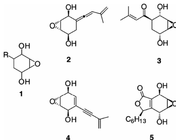
Figure 1. Naturally occurring epoxy-cyclohexane derivatives.
