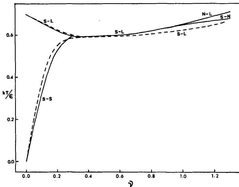
Figure 1. Reduced temperatures of solid-solid and melting transitions as functions of \nu ; — Present theory; --- Pople and Karasz. S-S Solid-solid, S-L Solid-liquid, S-N Solid-nematic, N-L Nematic-liquid transitions.
