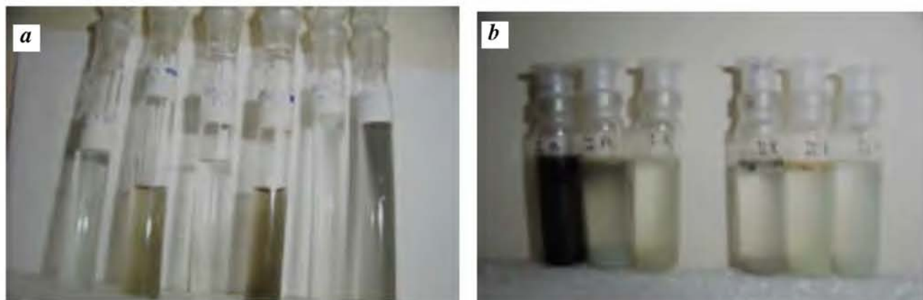
Figure 3. a (left and middle pair tubes) Salmonella and Proteus vulgaris , sulphide-yielding Enterobacteriaceae in modified bactosulphate API (SR)-soap medium (left tube, no growth) and in SIM medium (right tube, growth). (Right pair) Control tube and (extreme right), mud extract from Bhagwatghat tubewell-1 in modified sulphate API (SR)-soap medium. b , (left) Mud extract from Bhagwatghat tubewell-1 incubated with three different soap-containing modified sulphate API (SR)-soap medium. (Right) Mud extract from Bhagwatghat tubewell-2 after 7 days of incubation showing (cf. left panel) trace amounts of FeS precipitation.
