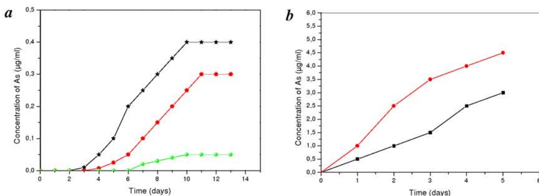
Figure 4. a , Arsenic releasing profile under SIM (black) and under modified soap medium (red), control (green); b , Dissolution profile of arsenic from pure As 2 S 3 (black) and FeS/As 2 S 3 (red) at pH 7. Data were average of three determinations from the same batch.
