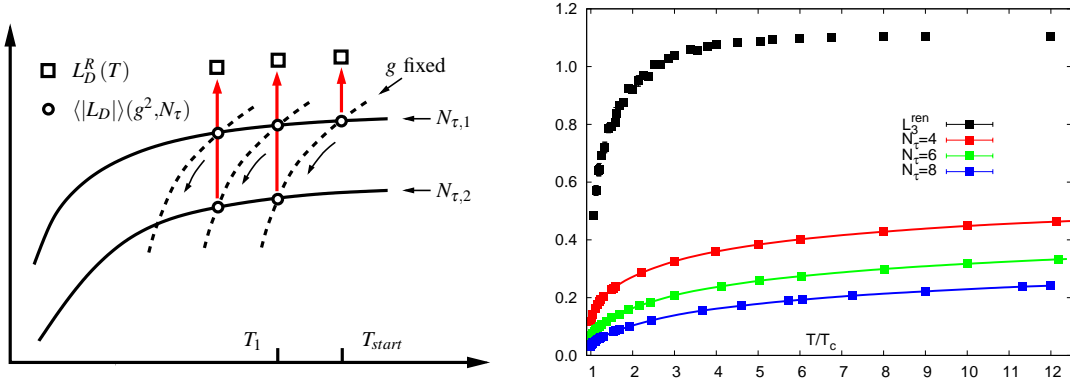
Figure 2: Renormalization procedure using different N_{\tau} (left). Bare Polyakov loops from 32^3 \times N_{\tau} lattices and the resulting L_3^{ren} . The lines are spline interpolations (right).
