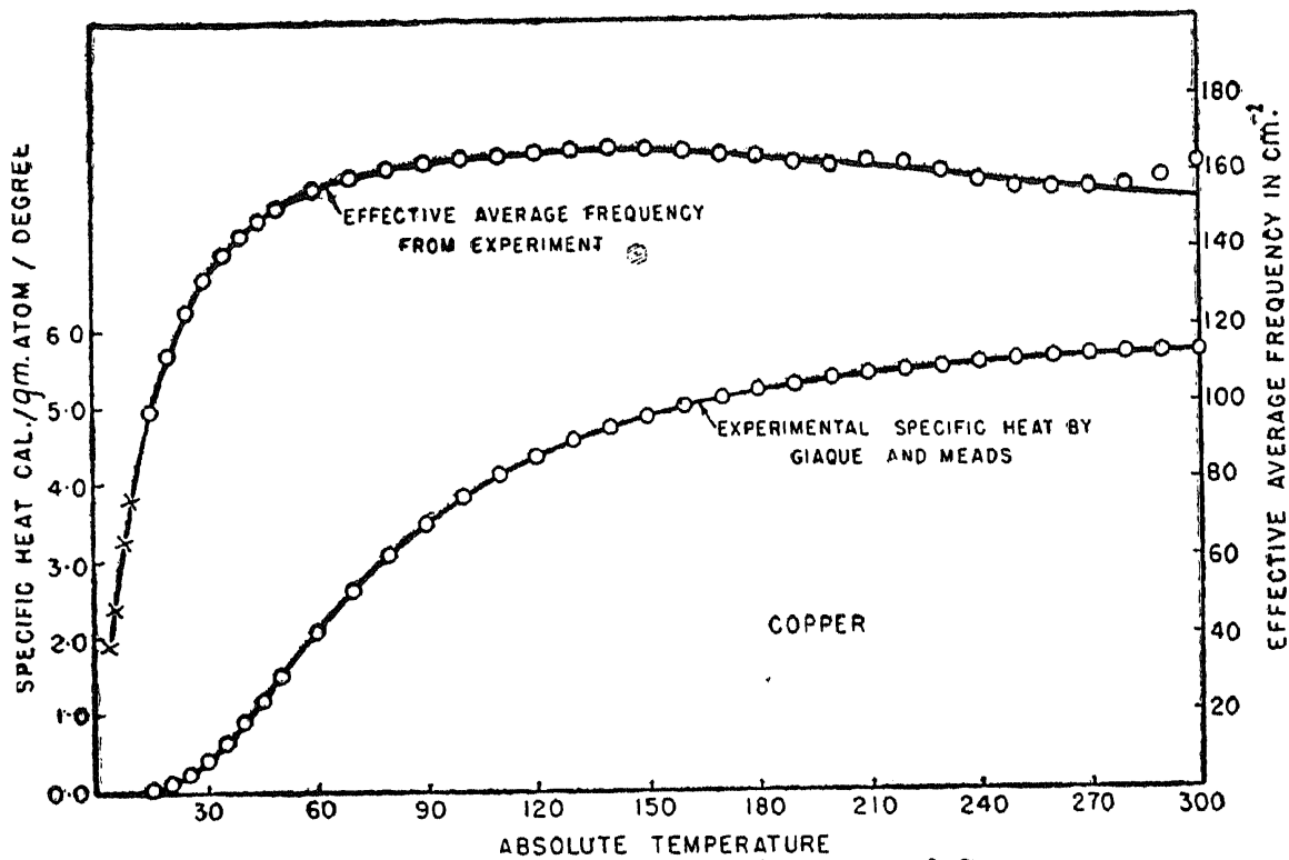
FIG. 2. Analysis of the Specific Heat of Copper.
