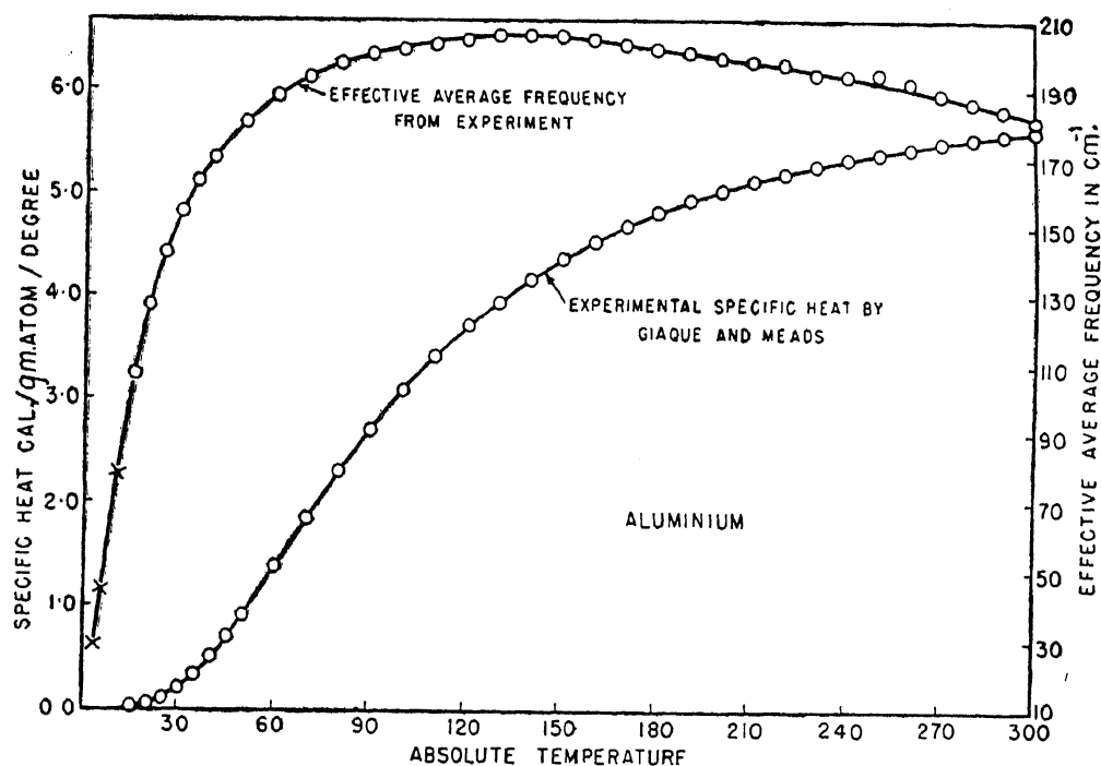
FIG. 1. Analysis of the Specific Heat of Aluminium.
