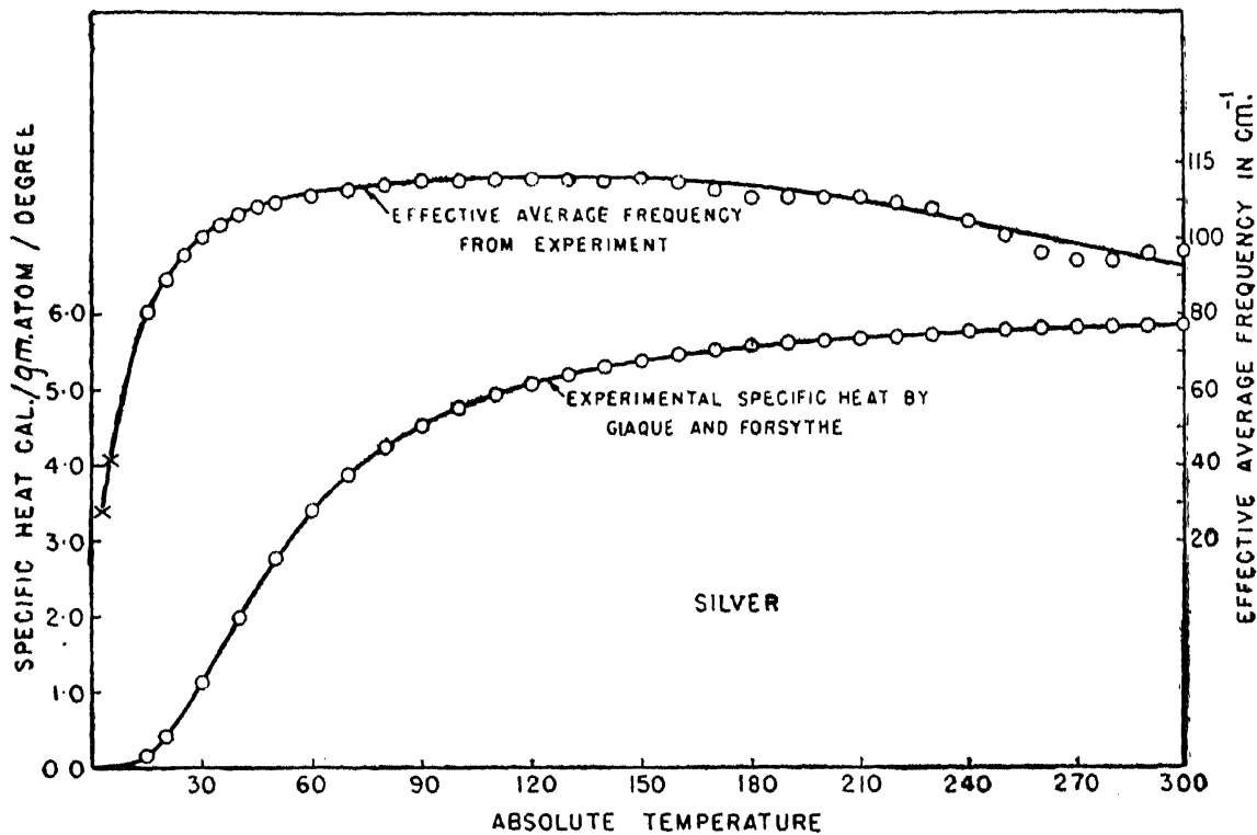
FIG. 3. Analysis of the Specific Heat of Silver.
