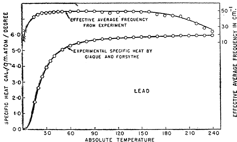
FIG. 4. Analysis of the Specific Heat of Lead.
