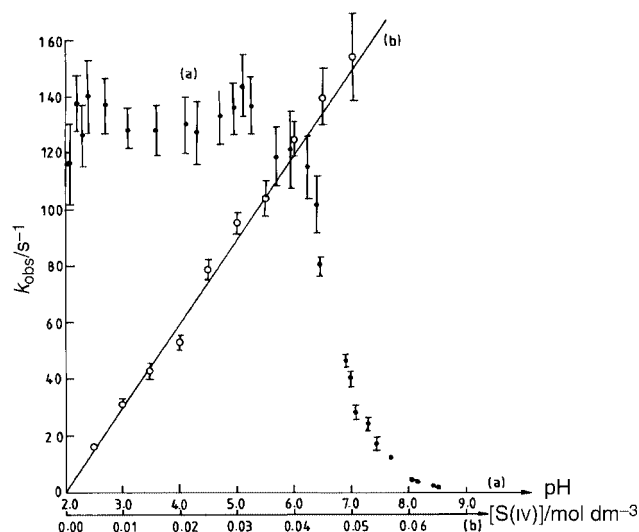
Fig. 6 (a) k_{\text{obs}}/\text{s}^{-1} vs. pH plot at [S IV ] T = 0.02 mol dm -3 and (b) k_{\text{obs}} vs. [S IV ] T /mol dm -3 plot at pH 6.6 for the formation of trans -[Co(salen)(OH 2 )(SO 3 -S)] - at 25.0 °C.
