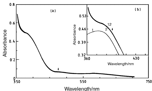
Fig. 4 Rapid scan spectra of trans -[Co(salen)(OH 2 ) 2 ] + + S IV at 25 °C. [Complex] T = 1.0 × 10 -4 + [S IV ] T = 0.02 mol dm -3 (pH 6.39, self buffered). (a) number of scans = 96, total time = 0.120 s; (b) inset: curve 1 for complex alone; curves 2–12 for the reaction mixture in 0.12 s; Δt = 0.012 s between successive runs.
