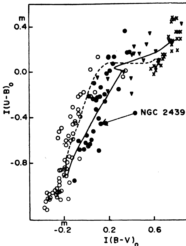
Figure 3. The I(U - B)_0 , I(B - V)_0 diagram. The notations are the same as in figure 2. Dashed curve represents the locus of the theoretical I(U - B)_0 , I(B - V)_0 curve calculated for the main sequence part of the cluster and the continuous curve represents the same curve calculated for the whole cluster (cf. Barbaro & Bertelli 1977).
