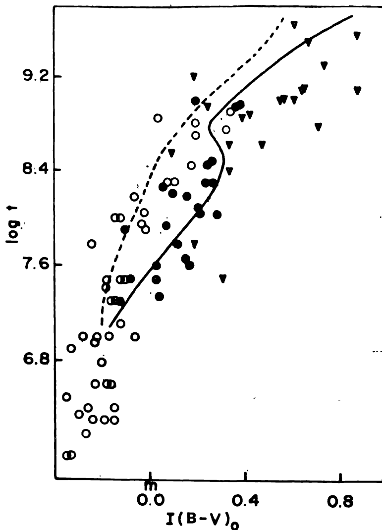
Figure 4. Plot of \log t versus I(B - V)_0 , where t is the age of the clusters in years. The notations are the same as in figure 2. Dashed and continuous curves represent the same curves as in figure 3.
