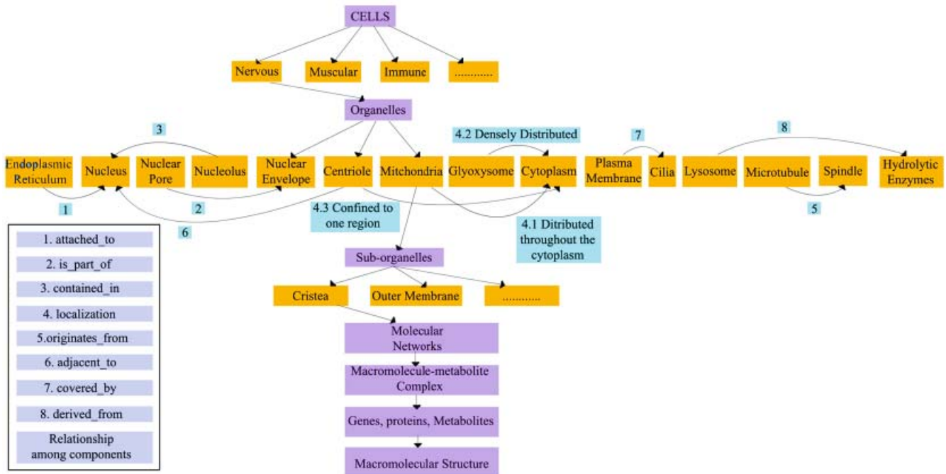
Figure 3. Improvised cell tree data-structure to store information about the cell. Application of scenegraph for cell modelling; the concepts of scenegraph and topological information lead us to extracting the substructure location information from cell images.
