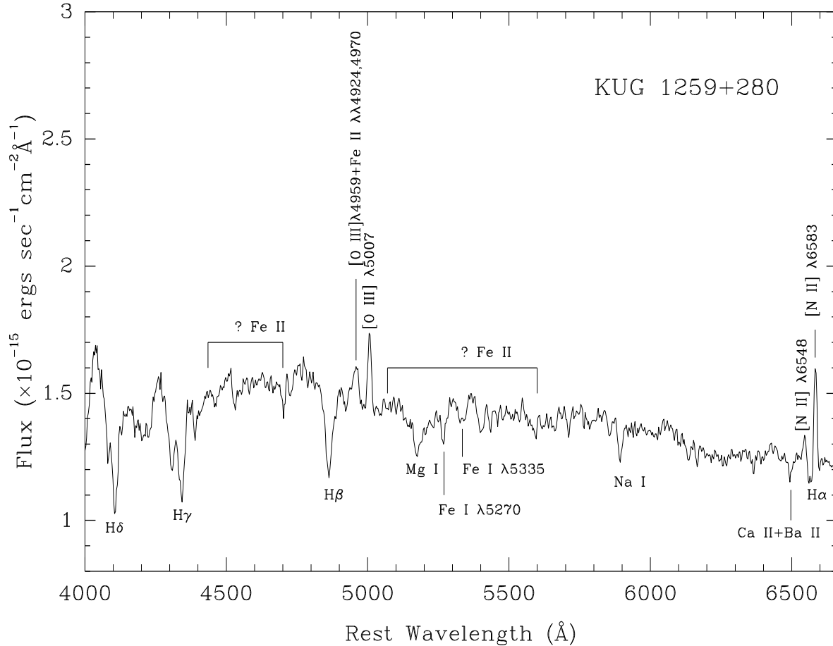
Figure 7. Doppler corrected and dereddened optical spectrum of KUG 1259+280. Balmer absorption line H\beta , H\gamma and forbidden emission lines e.g., [N II]\lambda 6583 , [O III]\lambda\lambda 4959, 5007 are seen clearly in the spectrum.
