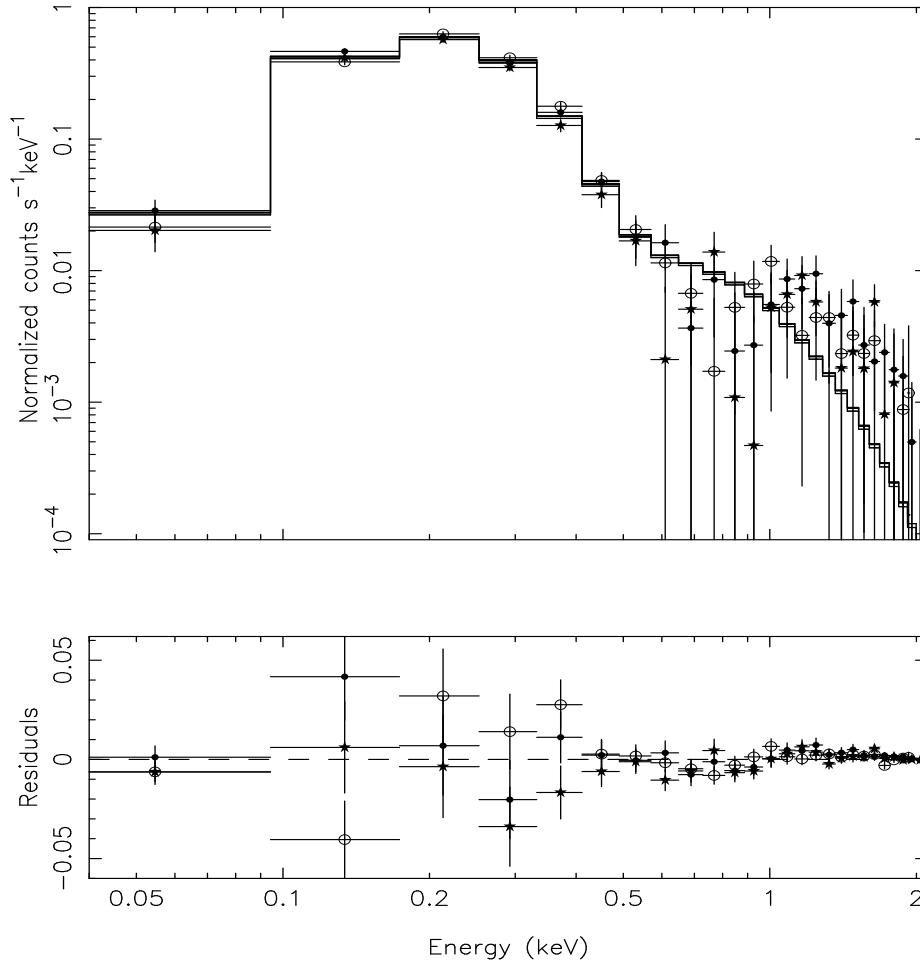
Figure 5. Spectral data and joint model fit to the ROSAT PSPC X-ray spectra of KUG 1259+280. The PSPC spectrum for 1991 June 16 observation is shown as solid circles. The spectrum marked with asterisks is for 1991 June 17 observation. The third spectrum marked with open circles is for 1991 June 18 observation. The jointly fitted power-law model absorbed by Galactic N_{\text{H}} and intrinsic N_{\text{H}} local to KUG 1259+280 is shown with solid line.
