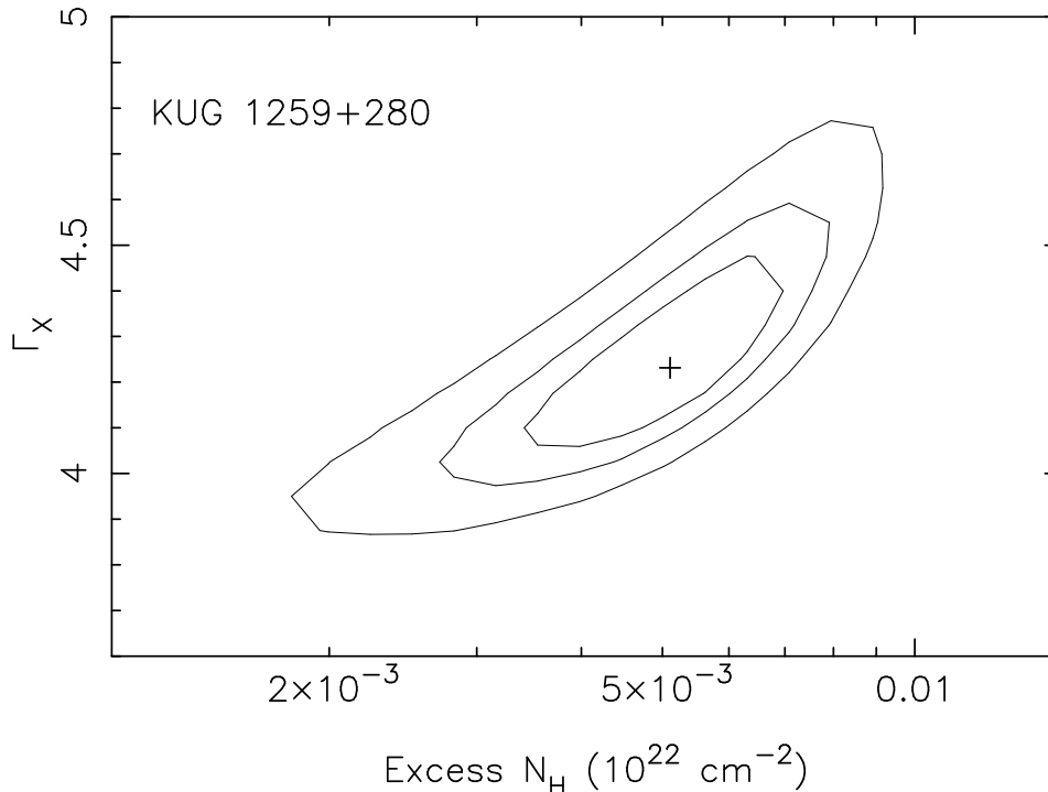
Figure 6. Allowed ranges of power-law photon index and ‘excess’ N_{\text{H}} (at the redshift of the source) for 68%, 90%, and 98% confidence based on counting statistics derived from the joint-fit of the 3 PSPC spectra. The ‘+’ marks the best-fit value.
