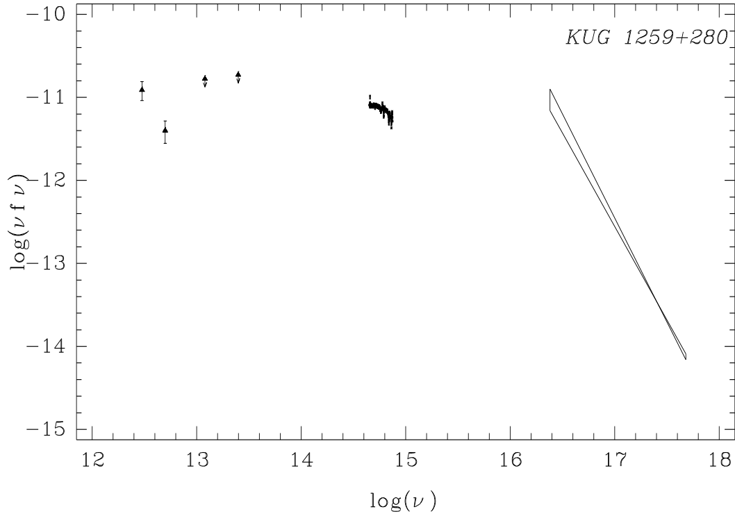
Figure 8. Spectral energy distribution of KUG 1259. Arrows indicate 3\sigma upper limits.
