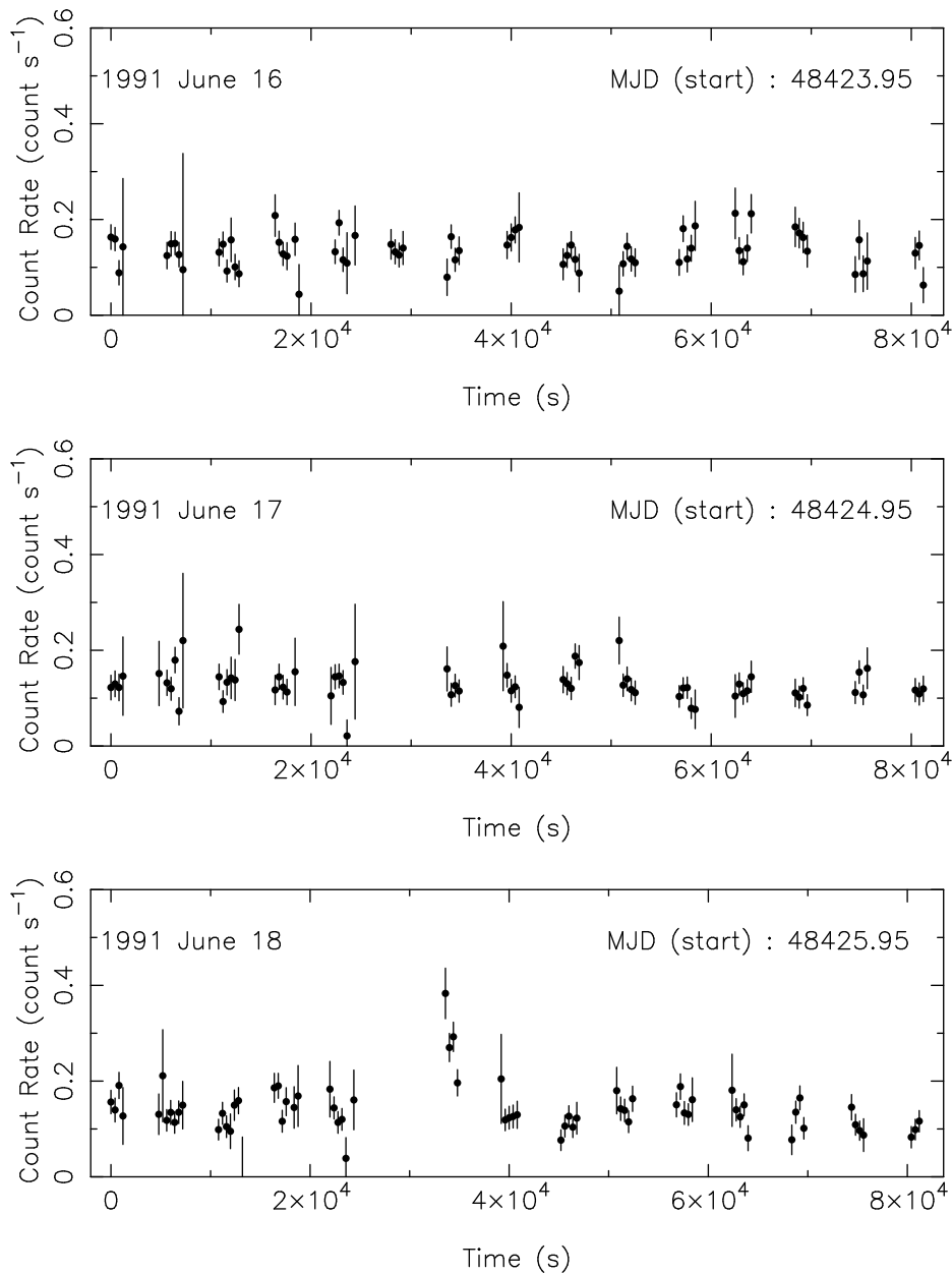
Figure 4. ROSAT PSPC light curves of KUG 1259+280 observed on (a) 1991 June 16, (b) 1991 June 17, and (c) 1991 June 18. The time bin size is 319 s. Short term variability is seen on 1991 June 18.
