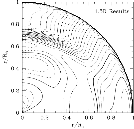
Figure 3. A contour diagram of the solar rotation rate as obtained by the 1.5D inversion technique using GONG months 4–14 data. Due to the symmetry of the inversion results, the rotation rate has been shown for just one quadrant only. The dotted contours have been drawn at intervals of 5 nHz., and the continuous ones at intervals of 20 nHz. The thick continuous line is the contour at a level of 440 nHz. The x -axis represents the solar equator while the y -axis represents the rotation axis.
