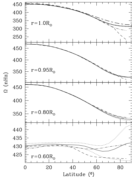
Figure 6. Comparison of the rotation inversion results at fixed radius. The line styles are the same as in Fig. 5. In the top panel the heavy short dashed- long dashed line shows the observed surface rotation rate as estimated by Doppler measurements (Snodgrass 1992).
