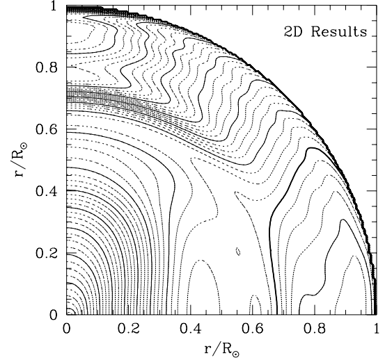
Figure 4. A contour diagram of the solar rotation rate as obtained by the 2D inversion of individual splittings using GONG months 4–14 data. The format is the same as that for Fig. 3.
