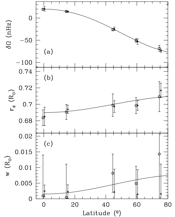
Figure 8. A summary of the tachocline results for the test model. Panels (a),(b) and (c) show the results of the jump, position and half-width respectively. In each panel the continuous line represents the exact value. The circles show the results of the calibration method and the triangles are the results obtained by 1D annealing. The symbols are displaced by \pm 0.5^\circ about the true latitude for the sake of clarity. In panel (c) the actual width has been scaled down by a factor of 3.25 to account for the difference in form of variation within the tachocline.
