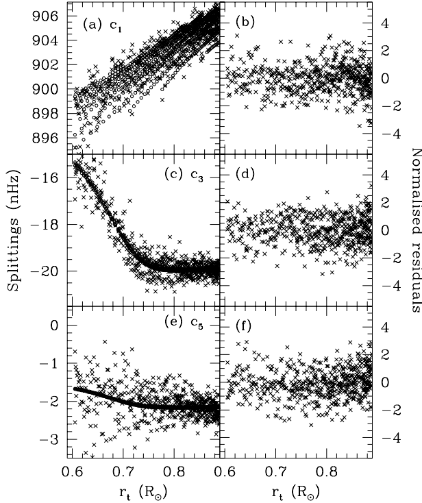
Figure 11. The fit to the first three splittings coefficients and the normalized residuals of the fits obtained by the 2D simulated annealing method assuming that there is no latitudinal variation in the position and thickness of the tachocline.
