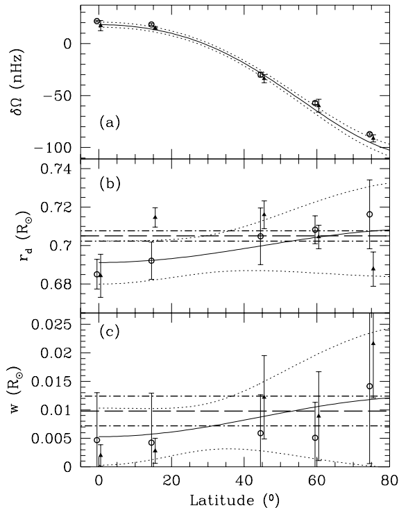
Figure 13. A summary of the tachocline results obtained using the GONG months 4–14 data. Panels (a),(b) and (c) show the results of the jump, position and thickness respectively. In each panel the continuous line is the results of the 2D annealing (equation 18) with the 1\sigma error bounds shown as the dotted lines. The circles show the results of the calibration method and the triangles are the results obtained by 1D annealing. The symbols are displaced by \pm 0.5^\circ about the true latitude for the sake of clarity. The dashed line in panels (b) and (c) mark the mean values found by Basu (1997), while the 1\sigma error bounds are shown as dot-dashed lines.
