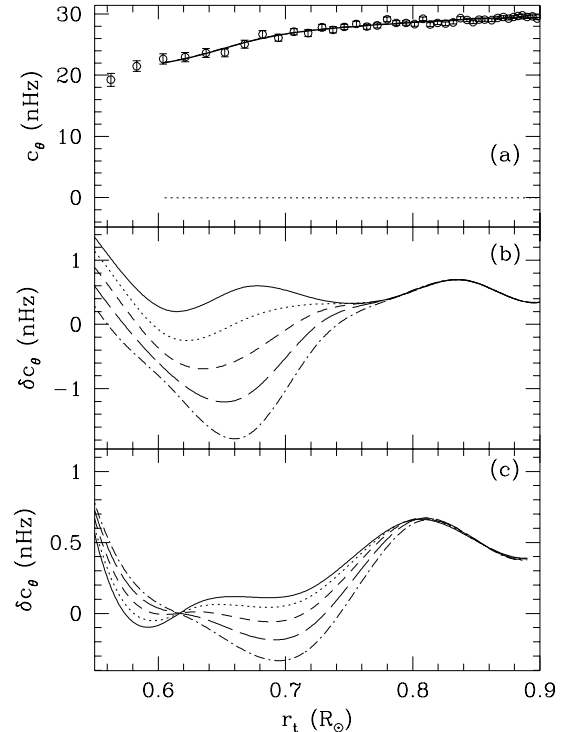
Figure 9. (a) Calibration for determining the jump in the rotation rate in tachocline. The points are the splitting-coefficients combination for the equator with the contribution from \Omega_c removed. The continuous line is the fit to the data, which can be decomposed into two parts — the dotted line which is the term \phi(r_t) in equation (13) and the dashed line which is the calibration model scaled to the fitted jump (term \alpha a_{\theta}(r_t) ). The data used are the GONG4–14 splittings. The dashed and continuous lines more or less coincide in this case. (b) The spline representation of the difference between the data shown above and the five calibration models used to determine the tachocline position. The continuous, dotted, small-dashed, long-dashed and dot-dashed lines are difference with calibration models for r_d = 0.68, 0.69, 0.70, 0.71 and 0.72R_{\odot} respectively. All these calibration models have w = 0.005R_{\odot} (c) The spline representation of the difference between the data and the five calibration models used to determine the tachocline width. The continuous, dotted, small-dashed, long-dashed and dot-dashed lines are difference with calibration models for w = 0.005, 0.01, 0.015, 0.02 and 0.025R_{\odot} respectively. These calibration models have r_d = 0.69R_{\odot} .
