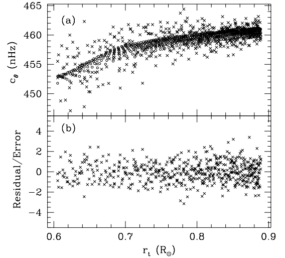
Figure 10. The 1D simulated annealing results for the solar equator. In Panel (a) The crosses are the observed splitting combinations and the circles are those obtained by the fit. Panel (b) shows the normalised residuals.
