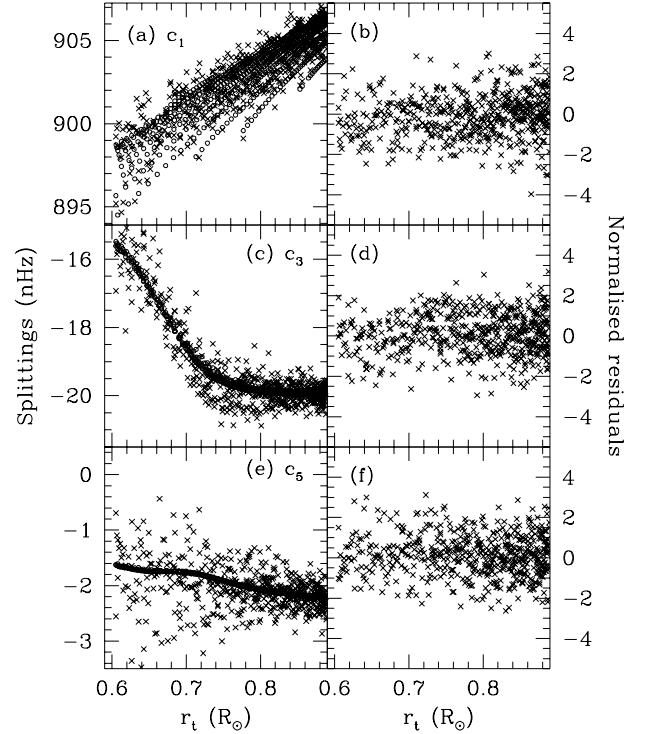
Figure 12. Same as Fig. 11, but with the possible latitudinal variation in the position and thickness of the tachocline taken into account
