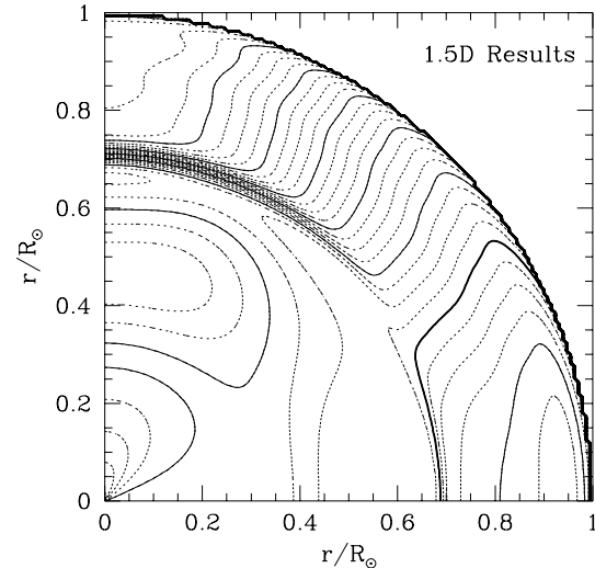
Figure 14. A contour diagram of the solar rotation rate as obtained by 1.5D inversion of the GONG months 4–14 data after removal of the tachocline. The format is the same as that for Fig. 3.
