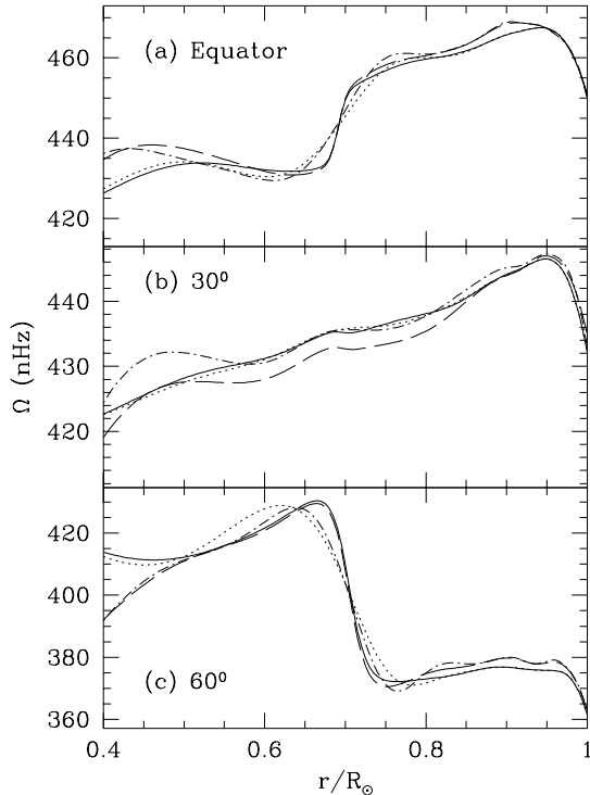
Figure 15. A comparison of the inversion results with and without removal of tachocline. Continuous line shows the results obtained using 1.5D inversion after removing the tachocline contribution, the dotted line is the 1.5D result of normal inversion. Similarly, the dashed line show the results of 2D inversion of individual splittings after removing the tachocline while the dot-dashed line shows the results from normal 2D inversion.
