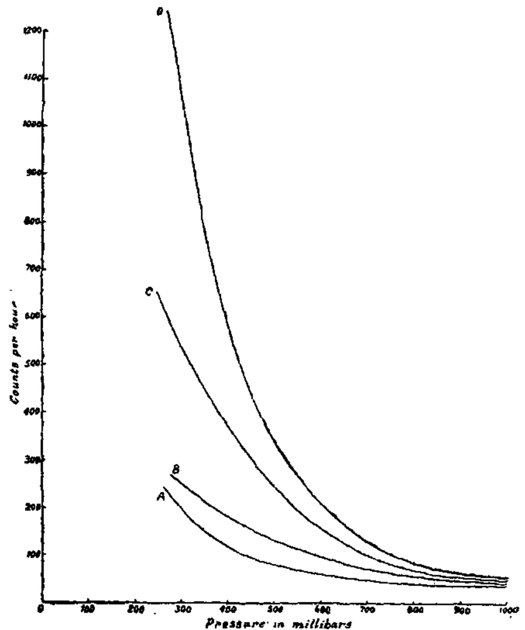
Curve A—Vertical meson intensity at 3.3^\circ N (Bhabha, Aiyar, Hoteko and Saxena). Curve B—Vertical meson intensity at 52.5^\circ N (Schein, Jesse and Wollan 1941). Curve C—Vertical total intensity at 3.3^\circ N (Neher and Pickering). Curve D—Vertical total intensity at 49^\circ N (Pfozter).
