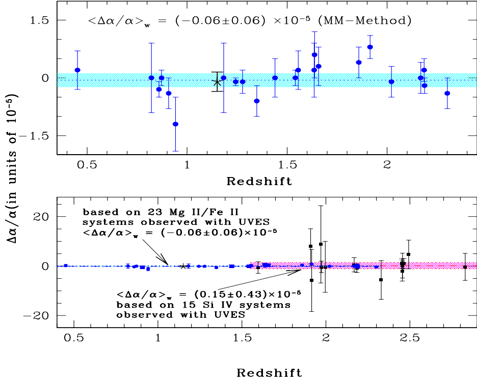
Figure 1. In the upper panel the results from the MM-method (using 23 Mg II/Fe II systems) are shown by filled circle. Shadow regions mark the 3\sigma range around the weighted mean. An asterisk (*) shows our preliminary result based on the analysis of Fe II multiplets in R \sim 100,000 spectrum of HE 0515-1444, obtained using HARPS. In the lower panel solid squares show the measurements using Si IV doublets (AD method). The measurements using the MM-method are also shown in this panel for comparison, by filled circles and the narrow shaded region.
