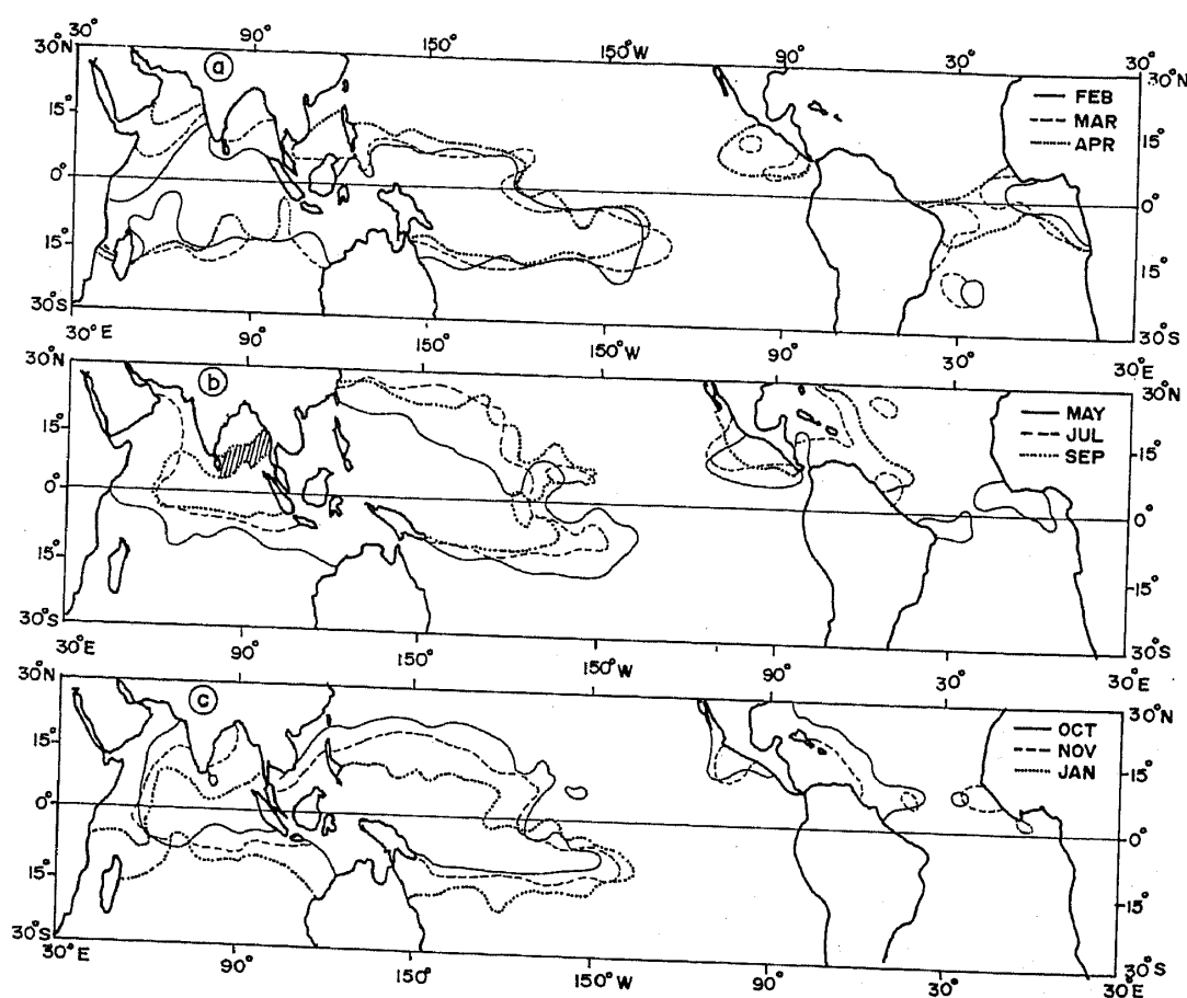
Figure 3. Annual evolution of the tropical warm pool. The contours show 28^{\circ}\text{C} isotherm during (a) February (—), March (---) and April (....); (b) May (—), July (---) and September (....); (c) October (—), November (---) and January (....). During September the warm pool in the Bay of Bengal is split into two parts separated by the shaded portion which is cooler.
