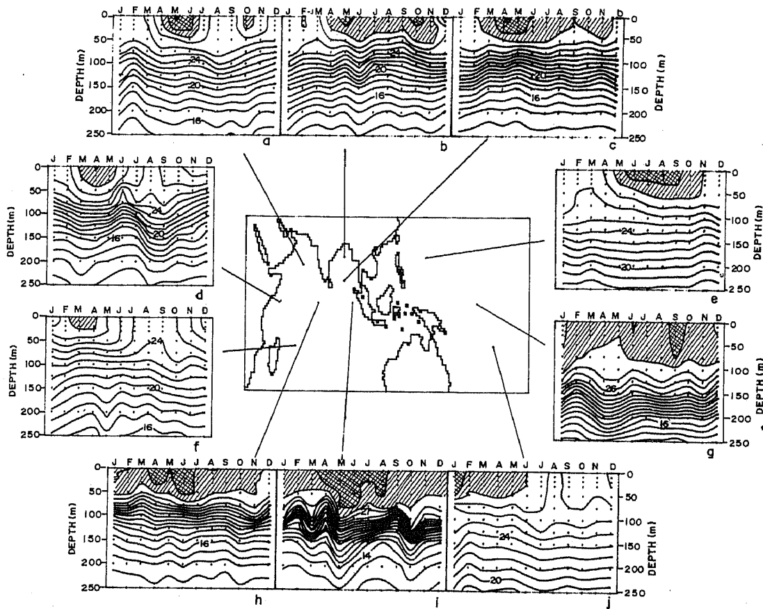
Figure 8. Annual cycle of thermal structure of the upper 250 m at selected locations. In the hatched, cross-hatched and shaded areas the temperature exceeds 28^{\circ}\text{C} , 29^{\circ}\text{C} and 30^{\circ}\text{C} respectively.
