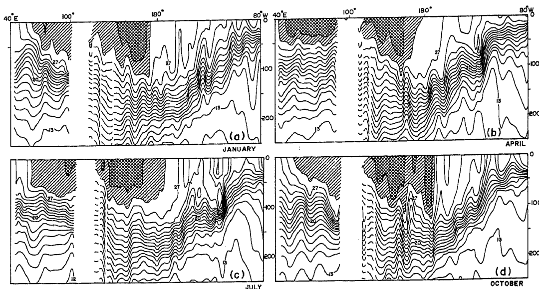
Figure 6. Vertical section of temperature along the equator from the east coast of Africa to Central America during (a) January, (b) April, (c) July, and (d) October. In the hatched, cross-hatched and shaded areas the temperature exceeds 28°C, 29°C and 30°C respectively. Vertical scale is in m.
