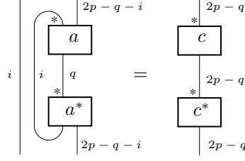
FIGURE 8. On positivity
