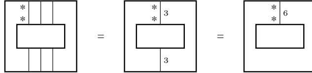
FIGURE 2. Illustration of cabling notation for tangles
