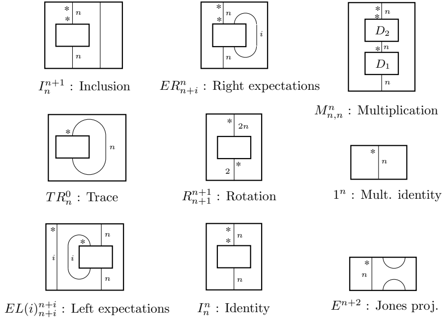
FIGURE 1. Some important tangles (defined for n \geq 0, 0 \leq i \leq n ).
