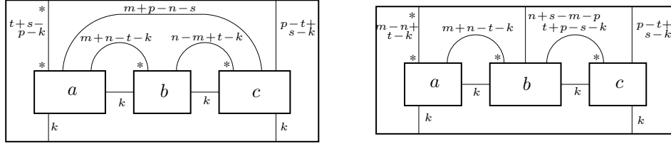
FIGURE 7. ((a\#b)\#c)_s = (a\#(b\#c))_u .
