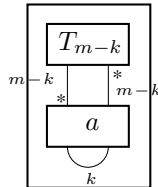
FIGURE 24. Definition of Tr_k(a) .
