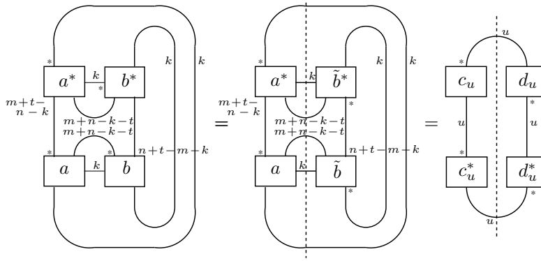
FIGURE 10. \delta^k \|(a\#b)_t\|_{H_k}^2
