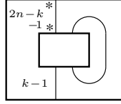
FIGURE 6. Definition of \delta E_{k-1} from P_n \subseteq F_k(P) to P_{n-1} \subseteq F_{k-1}(P) .
