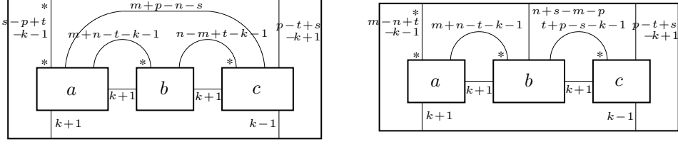
FIGURE 22. ((a\#b)_t.c)_s = (a.(b.c))_u .
