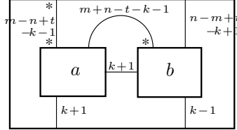
FIGURE 21. Definition of the P_t component of a \# b .
