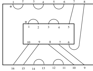
FIGURE 16. The tangle T(1, [4, 5], [3, 4])_8^8
