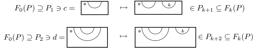
FIGURE 12. The elements c, d \in F_0(P) and their images in F_k(P)
