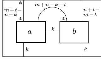
FIGURE 3. Definition of the P_t component of a\#b .
