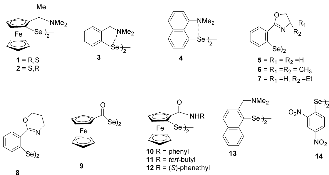
Chart 1. Diorganodiselenides as thiol peroxidase mimics.
