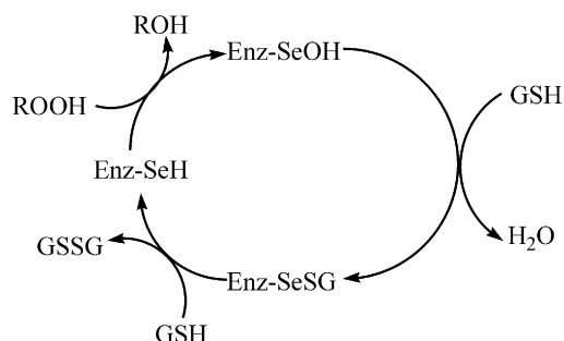
Scheme 1. Catalytic mechanism of glutathione peroxidase enzyme.
