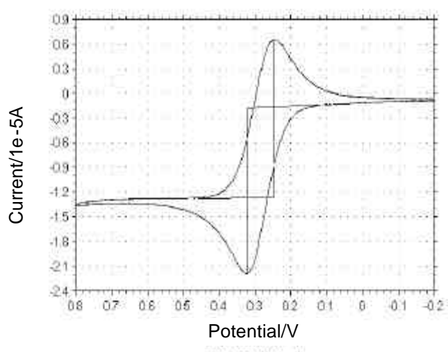
Figure 1. Cyclic voltammogram of compounds 10 .
