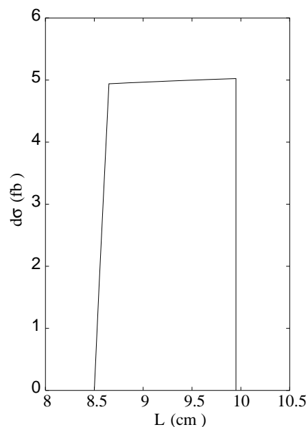
Figure 2: Chargino decay length distribution for the following set of input parameters: m_{3/2}=43 \text{ TeV} , m_0=230 \text{ GeV} , \tan \beta=3 , and \mu < 0 .
