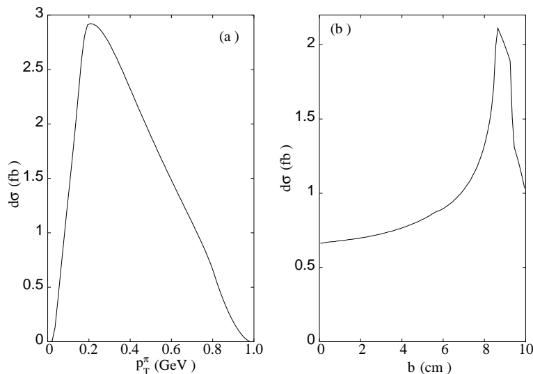
Figure 3: (a) Pion transverse momentum distribution and (b) the impact parameter distribution for the same set of input parameters as in figure 2.
