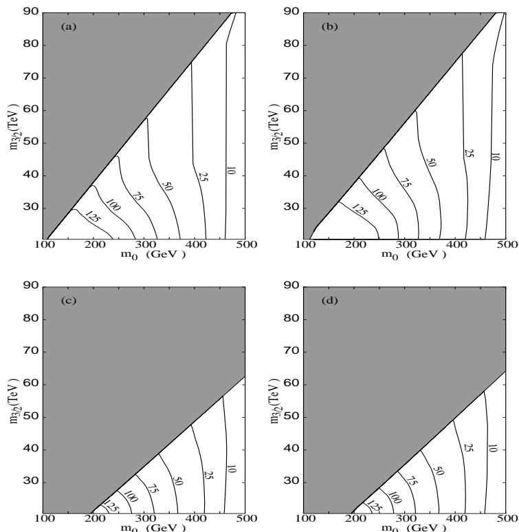
Figure 1: Constant cross section (in fb) contour plots in the m_0 - m_{3/2} plane for (a) \mu < 0 , \tan \beta = 3 , (b) \mu > 0 , \tan \beta = 3 , (c) \mu < 0 , \tan \beta = 30 and (d) \mu > 0 , \tan \beta = 30 .
