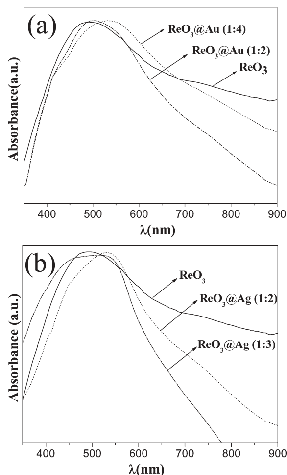
Fig. 5 UV-vis absorption spectra of (a) \text{ReO}_3@Au core-shell nanoparticles (1 : 2 and 1 : 4) with a 12 nm \text{ReO}_3 particle, and (b) \text{ReO}_3@Ag core-shell nanoparticles (1 : 2 and 1 : 3) with a 12 nm \text{ReO}_3 particle.
