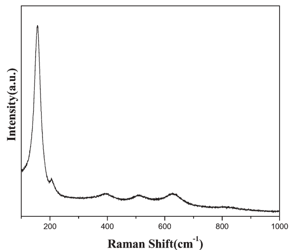
Fig. 8 Raman spectrum of \text{ReO}_3@TiO_2 core-shell nanoparticles.
