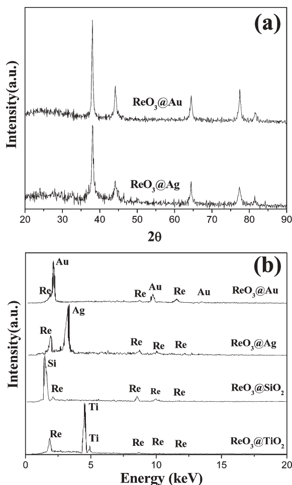
Fig. 4 (a) XRD patterns of \text{ReO}_3@Au and \text{ReO}_3@Ag core-shell nanoparticles, (b) EDAX spectra of \text{ReO}_3@Au , \text{ReO}_3@Ag , \text{ReO}_3@SiO_2 and \text{ReO}_3@TiO_2 core-shell nanoparticles.
