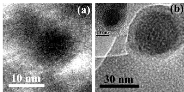
Fig. 6 (a) TEM image of a \text{ReO}_3@SiO_2 core-shell nanoparticle formed over an 8.5 nm \text{ReO}_3 particle, and (b) TEM image of a \text{ReO}_3@TiO_2 core-shell nanoparticle formed over a 32 nm \text{ReO}_3 particle with the inset showing a core-shell nanoparticle formed over a 12 nm particle of \text{ReO}_3 .
