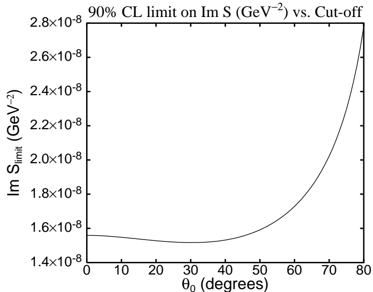
Figure 5: The 90% C.L. limit that can be obtained on \text{Im } S with an integrated luminosity of 500 \text{ fb}^{-1} plotted as a function of the cut-off angle \theta_0 .
