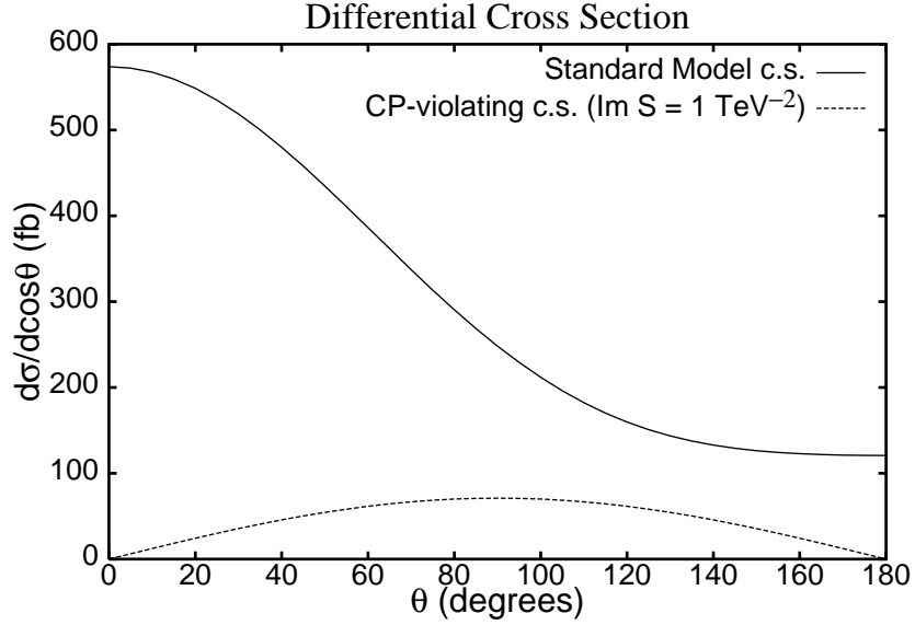
Figure 1: The SM differential cross section \frac{d\sigma}{d\cos\theta} (fb) (solid line) and the numerator of the asymmetry A(\theta) in eq. (8) (broken line) as a function of \theta . The latter is for \text{Im } S = 1 \text{ TeV}^{-2} .
