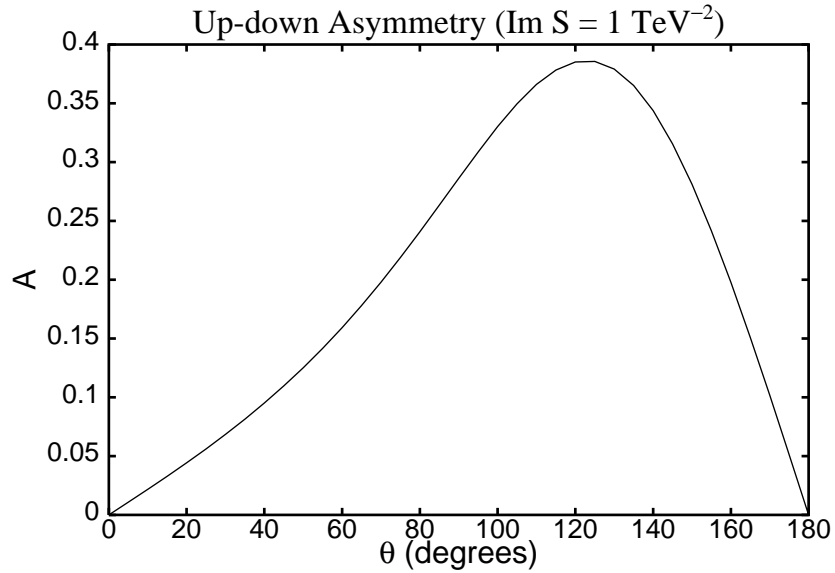
Figure 2: The asymmetry A(\theta) defined in eq. (8) as a function of \theta for a value of \text{Im } S = 1 \text{ TeV}^{-2} .
