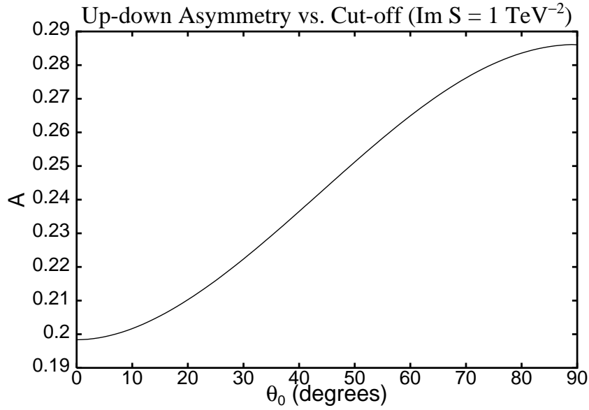
Figure 4: The asymmetry A(\theta_0) defined in eq. (9) plotted as a function of \theta_0 for \text{Im } S = 1 \text{ TeV}^{-2} .
