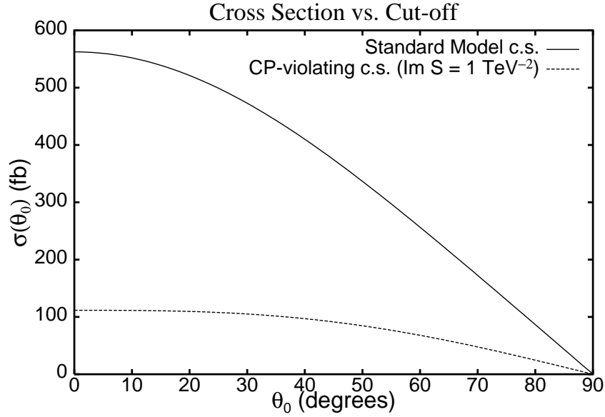
Figure 3: As in Fig. 1, but now for quantities integrated over \theta with a cutoff \theta_0 , plotted as a function of \theta_0 .
