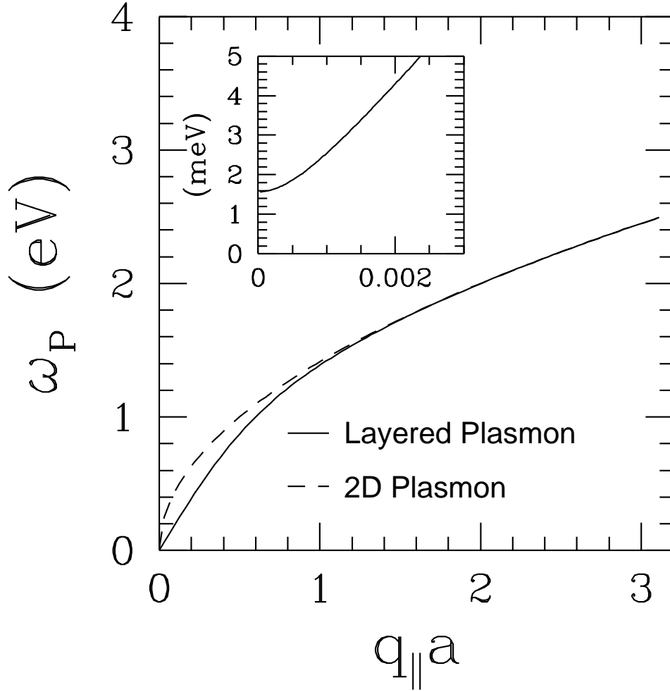
FIG. 1. The plasmon dispersion in a layered system (Bi2212), as a function of \mathbf{q}_{\parallel} with q_{\perp} = \pi/d_c (see text for details and parameters used). The \sqrt{q_{\parallel}} dispersion in the 2D limit is plotted for comparison. The dispersion appears nearly acoustic for small q_{\parallel} due to the very small Josephson plasma frequency ( \sim 10K ) but rapidly crosses over to high energies ( \sim eV ) with increasing q_{\parallel} . Inset shows the behavior of the dispersion (in meV ) for q_{\parallel} \rightarrow 0 .
