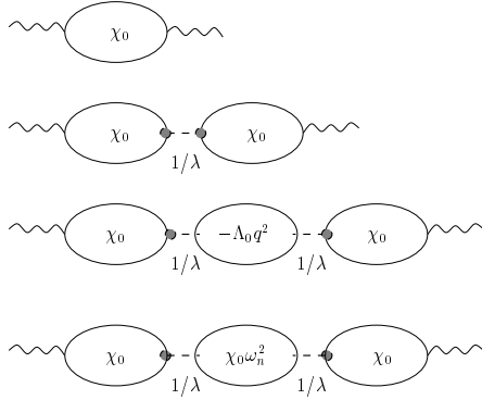
FIG. 3. Low order diagrams for \chi : The wavy lines indicate A_0 , the external scalar potential. The dashed lines contribute 1/\lambda , the “fake” \theta -propagator. The heavy dots refer to vertex factors of \omega_n arising from the vertex i\rho\partial_{\tau}\theta . Finally, the bubble contributions arising out of integrating out fermions are explicitly indicated.
