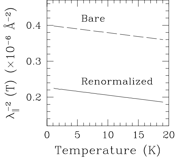
FIG. 2. The bare and renormalized 1/\lambda_{\parallel}^2 plotted as a function of temperature near optimal doping for Bi2212. We have chosen bare values such that the renormalized results, \lambda_{\parallel}(0) \approx 2100\text{\AA} and d\lambda_{\parallel}/dT \approx 10.0\text{\AA}/K , are in approximate agreement with experiment.
