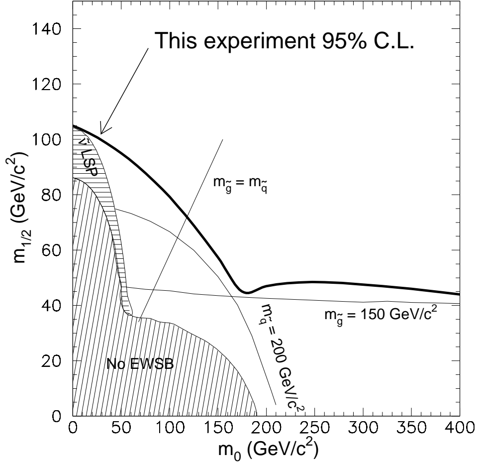
FIG. 2. Exclusion contour in the (m_0, m_{1/2}) plane for A_0 = 0 , \mu < 0 , \tan \beta = 6 , and a finite \lambda'_{1jk} ( j=1, 2 and k=1, 2, 3 ) coupling.
