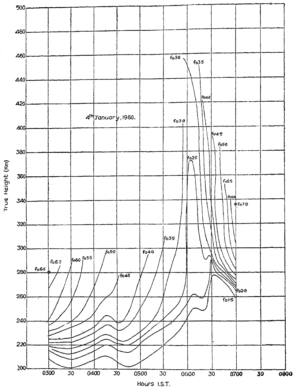
FIG. 4. Height variations of constant ionization levels of January 4, 1960, during pre-sunrise F-region "splitting".
