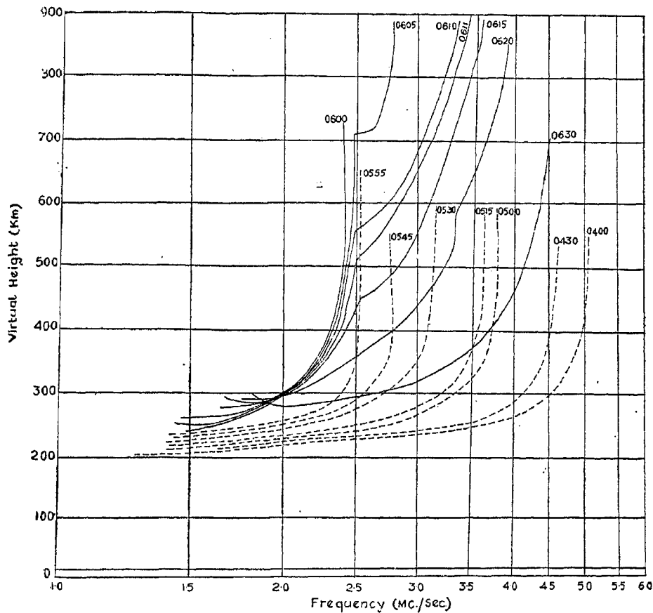
FIG. 2. Ordinary component of the h' - f traces between 0400 hr. and 0630 hr. I.S.T. on January 4, 1960.
