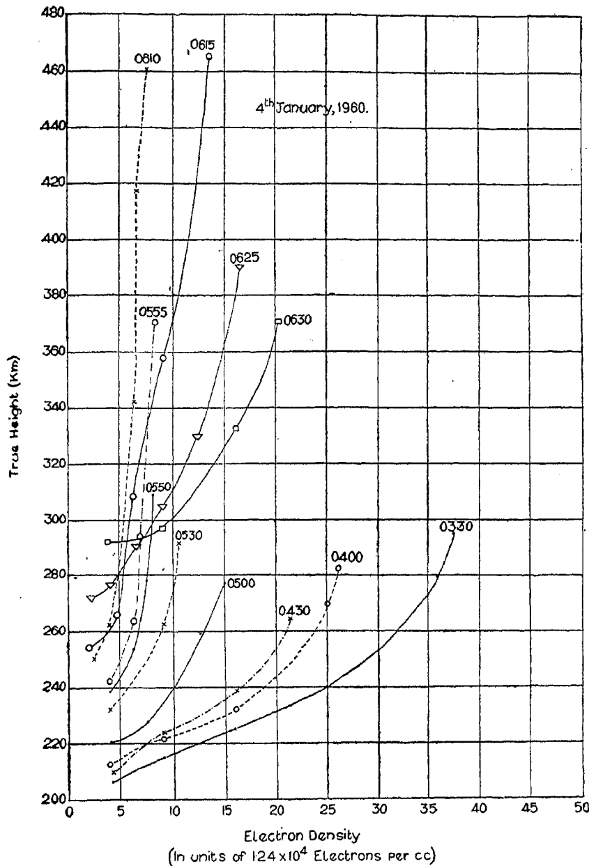
FIG. 3(b). (N, h)_f profiles between 0330 hr. and 0630 hr. I.S.T., deduced from h'f records of January 4, 1960.
