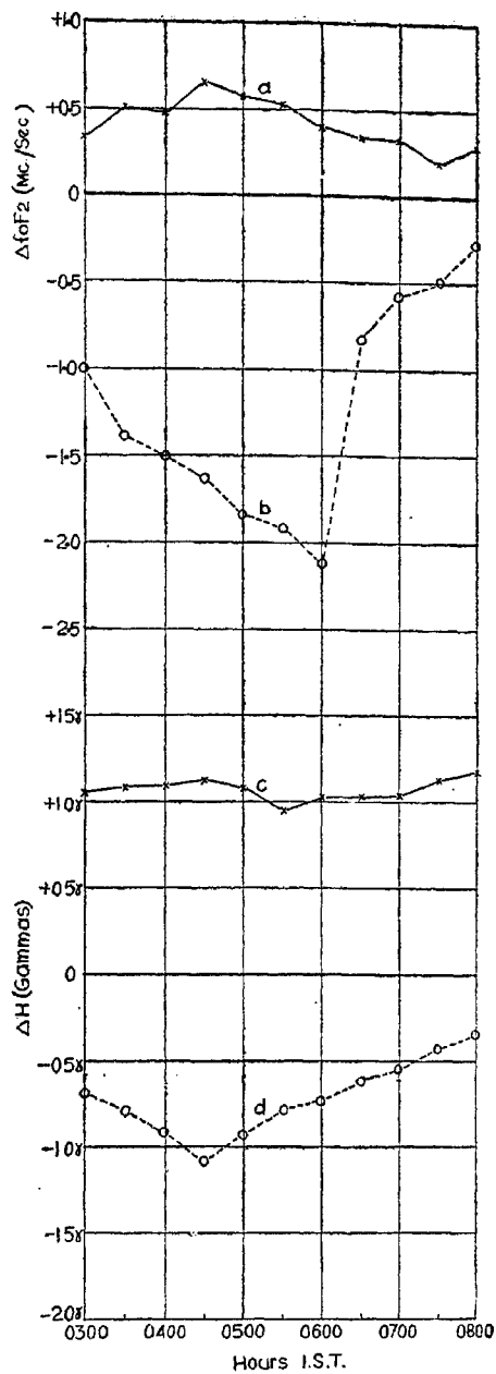
FIG. 5. Upper curves: Variation of \Delta foF_2 for January 1960: (a) for 21 days when pre-sunrise minimum of foF_2 was > 3.0 Mc./sec. and (b) for 9 days when the parameter was found to be \leq 3.0 Mc./sec.
