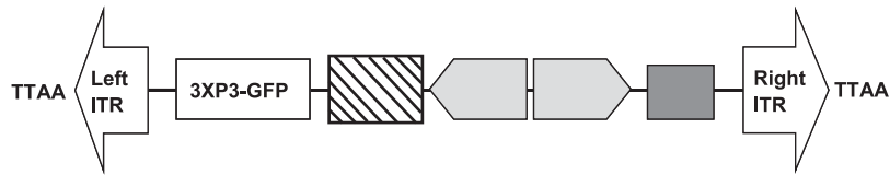
Figure 1. PiggyBac -based RNAi vector, pPIG3XP3-GFP-FF (11 kb) used for constructing transgenic silkworms with 3XP3-GFP gene as a selection marker. Left ITR and Right ITR indicate left and right terminal inverted repeats, respectively. ie-1FF cassette (light grey boxes) comprises 630 bp of ie-1 promoter (hatched box), 470 bp of ie-1 gene fragment in 'flip-flop' orientation and 200 bp polyadenylation signal (dark grey box). The construct pPIGA3GFP-FF that was used for cell culture assays had the A3-GFP cassette instead of the 3XP3-GFP cassette.
