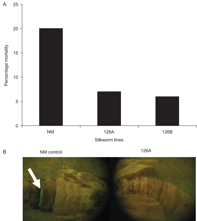
Figure 6. (A) BmNPV resistance in transgenic pupae injected with budded virus. Pupae from two transgenic lines and the control NM line were injected with free virus at a dose of 60 BV/pupa. The result indicates threefold reduced viral induced mortality in transgenic line 126A and 126B, confirming antiviral property conferred by the transgene. (B) Stereomicroscope micrograph of intact nontransgenic and a transgenic moths emerged from the pupae injected with a recombinant GFP expressing BmNPV, BmNPV-P10GFP . The white arrow points to GFP expressed from BmNPV, which is found predominantly in the nontransgenic NM control line compared with the transgenic 126A line.
