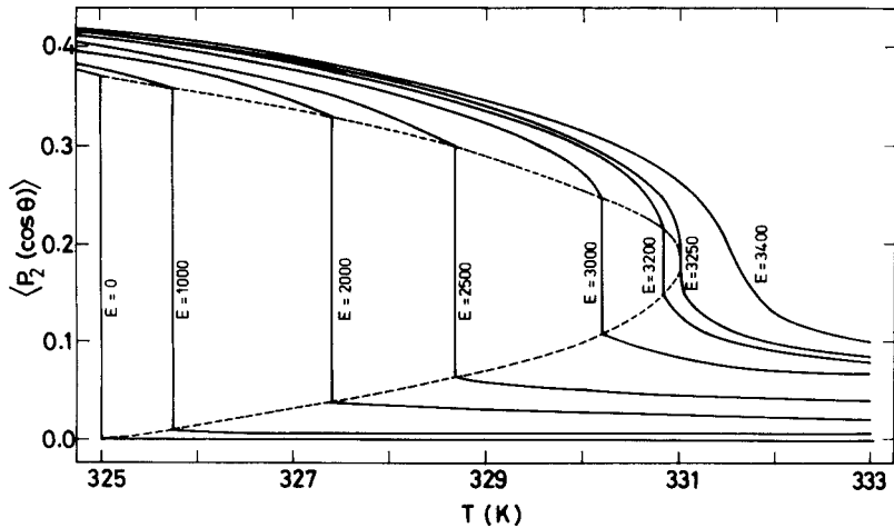
FIGURE 2 Variation of \langle P_2(\cos \theta) \rangle as a function of temperature T for various values of the electric field E .
