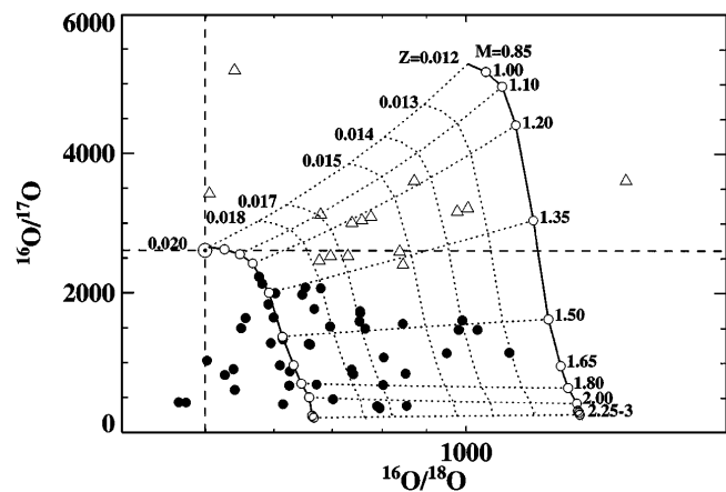
FIG. 2. Comparison of oxide grain data for groups 1 and 3 (see Fig. 1 for symbol definitions) with predictions of O-isotopic ratios following first dredge-up in red giant stars of initial mass (0.85\text{--}3)M_{\odot} and metallicity Z = 0.012\text{--}0.02 [22]. For the sake of clarity, error bars on grain measurements are not shown. Each open circle corresponds to predictions for a distinct star. The dotted lines indicate interpolated values for masses and metallicities intermediate to those calculated. Oxide grains belonging to groups 1 and 3 have isotopic compositions consistent with these predictions, provided that they come from several different stars with distinct masses and initial compositions.
