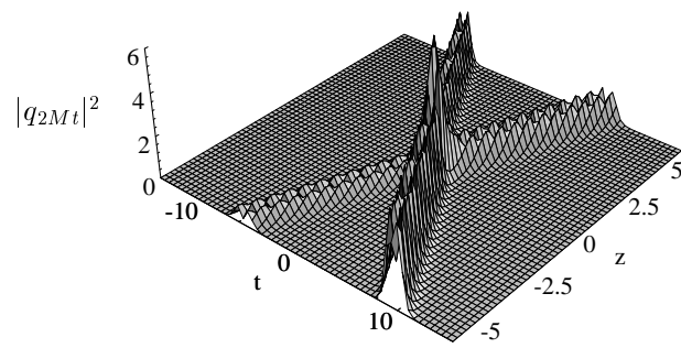
FIG. 3. Intensity profiles |q_{1Mt}|^2 and |q_{2Mt}|^2 of the two-soliton solution of the Manakov model with the parameteric values as in Fig. 2
