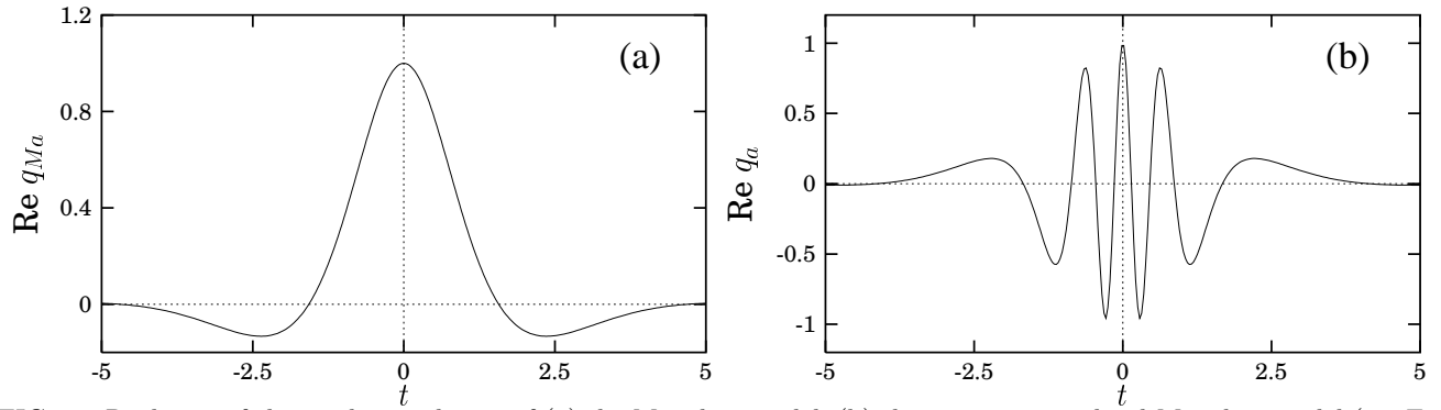
FIG. 1. Real part of the 1-soliton solution of (a) the Manakov model, (b) the quintic generalized Manakov model (see Eqn. (18)).
