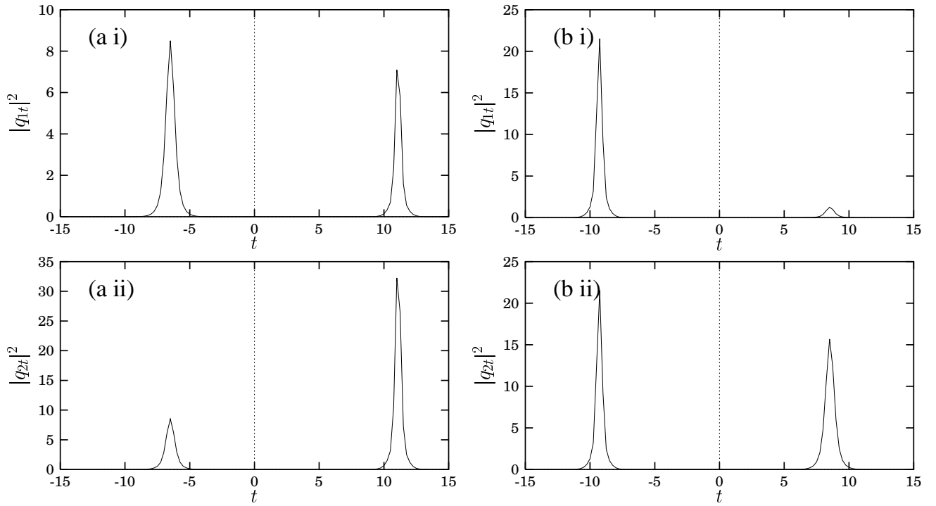
FIG. 4. Asymptotic forms of the intensity profiles |q_{1t}|^2 and |q_{2t}|^2 of the two-soliton solution (19) of the generalized model (9), (a) at z = -7 , (b) z = +7 , for nonzero values of the parameters \rho_1 = \rho_2 = \tau_1 = \tau_2 = 1 and with remaining parameters as in Fig. 3. Note the suppression of the soliton splitting, which appeared in the asymptotic profile in Figs. 2 and 3.
