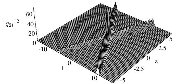
FIG. 5. Intensity profile |q_{1t}|^2 and |q_{2t}|^2 of the two-soliton solution (19) of the generalised Manakov model with the parameter values as in Fig. 4. Note the persistence of inelastic soliton collision as in the Manakov model and a higher intensity of modes during soliton interaction compared to the Manakov model.
