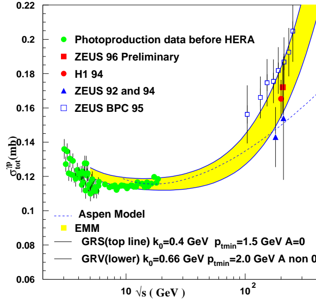
FIGURE 3. Comparison between the eikonal minijet model predictions and data for total \gamma p cross-section as well as BPC data extrapolated from DIS [15]. Predictions from [17] are also shown.
