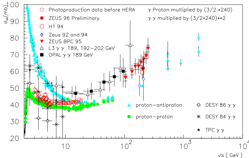
FIGURE 1. Energy dependence of \sigma_{ab}^{\text{tot}} for various choices of a, b as indicated in the figure. The cross-sections for the photon-induced processes have been scaled as indicated on the figure.
