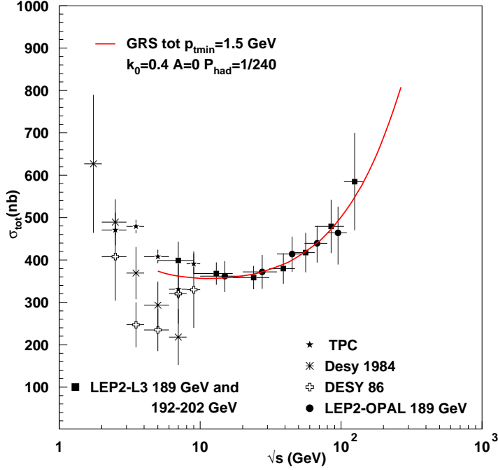
FIGURE 2. The total photon-photon cross-section as described by the EMM (see text)
