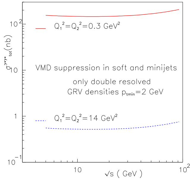
FIGURE 4. The EMM predictions for virtual photons cross-section. Q_i^2 corresponds to the virtual photon mass
