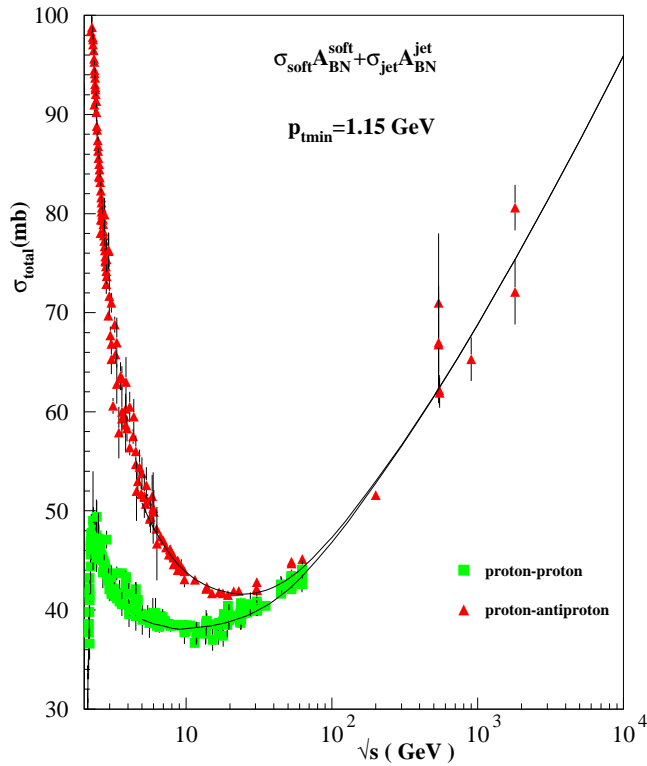
FIGURE 5. Total proton-proton and proton-antiproton cross-sections, compared with an eikonal minijet model which incorporates soft gluon summation
