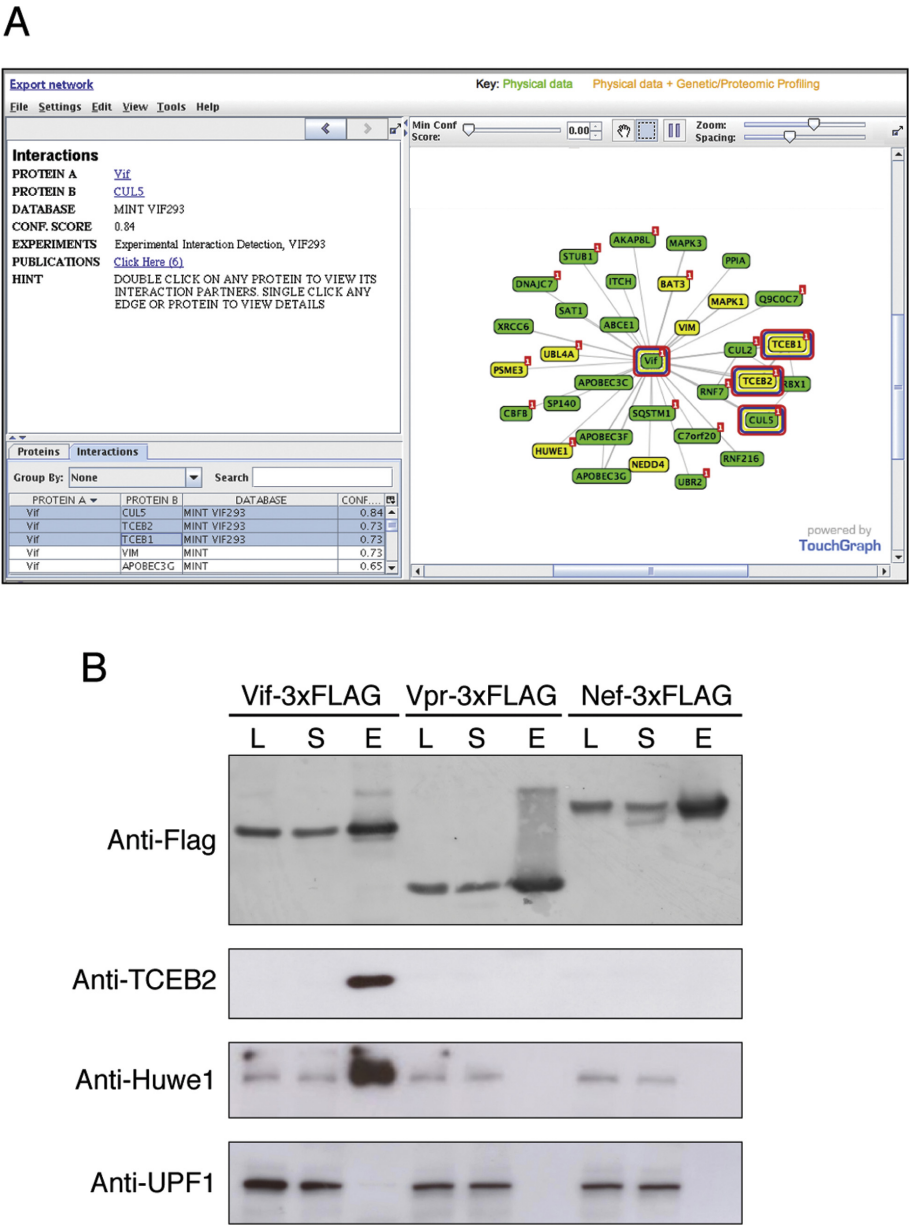
Figure 5 User-generated data can be uploaded and viewed in the context of complete PPI networks from public databases. (A) Vif network from GPS-Prot, including an uploaded dataset from AP-MS experiments (red-tagged nodes). Huwe1 is among several proteins in the uploaded dataset (Jager et al., submitted) that are not found in other databases (e.g., not present in Figure 2B), and were also previously identified by genetic/proteomic screens. (B) HIV Vif interacts with endogenous HUWE1 in 293 cells. 3xFLAG-tagged Vif, Vpr, and Nef were immunoprecipitated with anti-FLAG agarose beads. Lysates (L), remaining supernatant (S) and eluates (E) were analyzed by SDS-PAGE and Western blotting with antibodies as indicated. The same band is identified in the Vif pulldown by antibodies against the known CUL5 E3 ligase complex, anti-CUL5 (not shown) and anti-ELOB (TCEB2) as well as anti-Huwe1 antibodies, but not by the control anti-UPF1 antibody.
