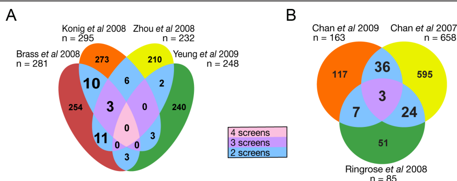
Figure 1 Numerous host factors have been identified for HIV by small-scale and high-throughput experiments, with little overlap between the various sources. (A) Venn diagram shows overlap from four HIV-based genetic screens [14-17]. Only three intersections show a significantly higher number of shared genes than expected, which are highlighted in large type. Ten genes are shared between the Brass and König datasets ( p = 0.01 ), 11 between Brass and Zhou datasets ( p = 0.0014 ), and three between Brass, König, and Zhou datasets ( p = 5 \times 10^{-5} ). None are shared between all four datasets. (B) Venn diagram shows a similar analysis for three HIV-dependent proteomic profiling screens [26-28]. Large type highlights statistically significant overlaps between the datasets (below 1 \times 10^{-4} ).
