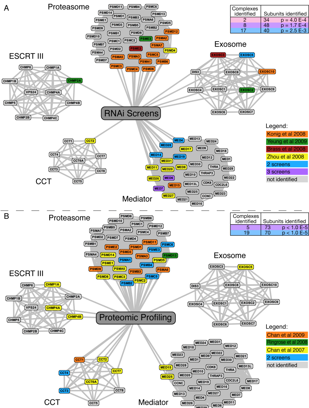
Figure 4 Five complexes implicated in HIV pathogenesis by analysis with CORUM. (A) Network analysis of RNAi datasets. Gray nodes are subunits present in the complex according to the CORUM database. Colored subunits (nodes) were reported in one or more of the genetic screens. Based on the hypergeometric distribution, we find significantly more subunits of the proteasome ( p = 4.2 \times 10^{-9} ), Mediator ( p = 1.1 \times 10^{-9} ), and the exosome ( p = 2.1 \times 10^{-3} ) than expected. Subunits of ESCRT III and CCT complexes are not significantly enriched. The table shows the number of complexes and subunits identified by two, three or four RNAi screens. As with genetic screens, there is greater overlap between datasets when analyzed in terms of subunits of complexes as opposed to isolated proteins. (B) Network analysis of proteomic profiling datasets. The same complexes are shown as in panel A, with subunits highlighted as they occur in different datasets. Mediator and exosome complexes are not covered more than expected, but significantly more subunits than expected are found for ESCRT III ( p = 8.4 \times 10^{-3} ) and CCT complexes ( p = 2.0 \times 10^{-7} ). The proteasome is the only complex where more subunits than expected are identified by both genetic and proteomic profiling screens ( p = 7.0 \times 10^{-23} ).
