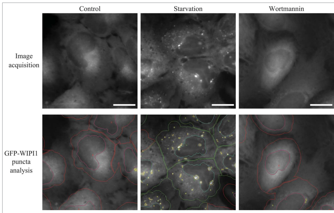
Figure 18. Automated WIPI1 puncta image acquisition and analysis monitors the induction and inhibition of autophagy. Stable U2OS clones expressing GFP-WIPI1 were selected using 0.6 \mu g/ml G418 and then cultured in 96-well plates. Cells were treated for 3 h with nutrient-rich medium (control), nutrient-free medium (EBSS), or with 233 nM wortmannin. Cells were fixed in 3.7% paraformaldehyde and stained with DAPI (5 \mu g/ml in PBS). An automated imaging and analysis platform was used to determine the number of both GFP-WIPI1 puncta-positive cells and the number of GFP-WIPI1 puncta per individual cell. 470 Cells without GFP-WIPI1 puncta are highlighted in red (cell detection) and purple (nuclei detection), whereas GFP-WIPI1 puncta-positive cells are highlighted in yellow (GFP-WIPI1 puncta detection), green (cell detection) and blue (nuclei detection). Scale bars: 20 \mu m. Images provided by S. Pfisterer and T. Proikas-Cezanne.
