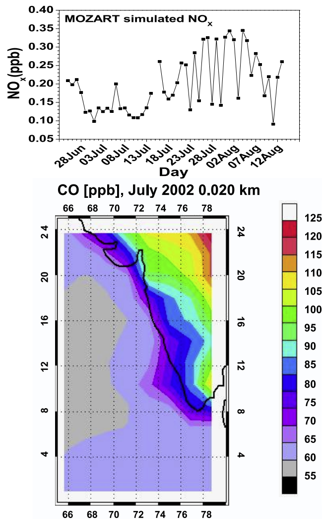
Figure 4. (top) Time series of daily average value of NO_x over the Arabian Sea during ARMEX 2002 and (bottom) average spatial variation of CO during July 2002.
