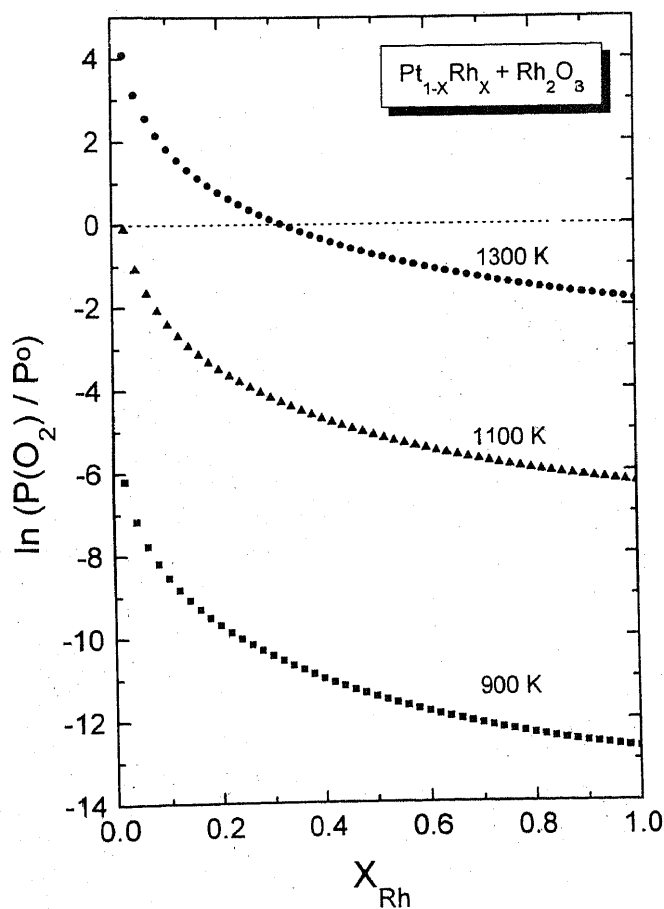
Figure 2. Variation of the equilibrium oxygen chemical potential for the formation of \text{Rh}_2\text{O}_3 as a function of composition of Pt-Rh alloys at different temperatures.
