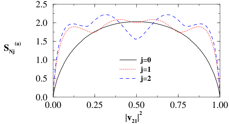
Figure 1: Plot of S_{Nj}^{(a)} as a function of |v_{21}|^2 for N = 4 and j = 0, 1, 2 .
