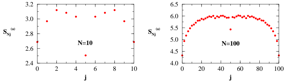
Figure 2: Plot of S_{Nj}^{(a)} as a function of j for |v_{21}|^2 = 1/2 and a given total number of photons N .
