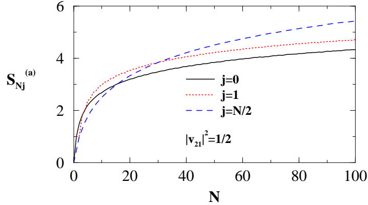
Figure 3: Plot of S_{Nj}^{(a)} as a function of N for |v_{21}|^2 = 1/2 and j = 0, 1, N/2 .
