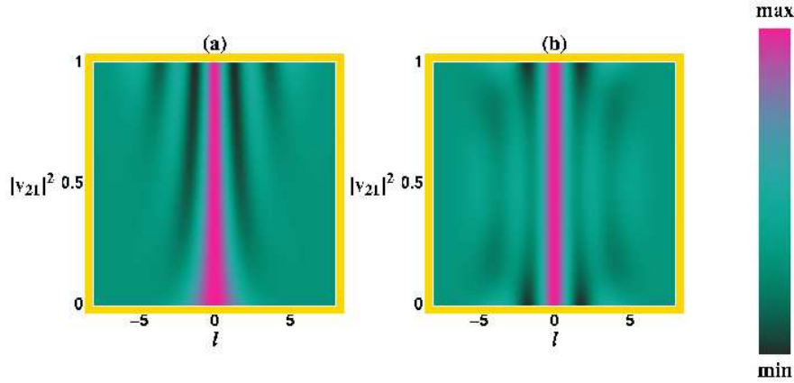
Figure 6: Contour plot of \gamma_{Nj}^{(a)}(l) as a function of l and |v_{21}|^2 when N = 4 and j = 0 (left), j = 2 (right).
