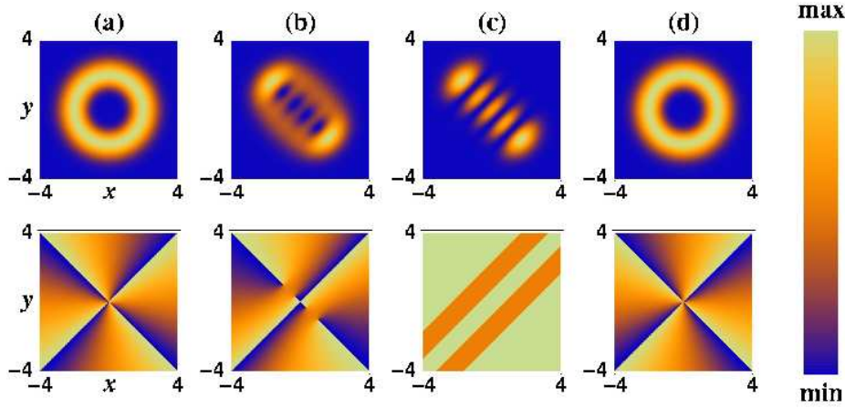
Figure 4: Time evolution of an initial vortex state for \Theta = 0 even though the entropy \tilde{S}_{Nj}^{(a)} remains constant. Shown here are the contour plots of the absolute square (top row) and the phase (bottom row) of \tilde{\psi}_{Nj}(x, y, t) as functions of x and y at different times with b_{Nj}^{(n)} as given in (60). Here, N = 4 , j = 0 and \cos^2 \Omega t has the values (a) 1.0, (b) 0.9, (c) 0.5 and (d) 0.0. The horizontal and the vertical axes refer to the x and y coordinates respectively. For the phase plots, we have used the convention that the phase ranges from -\pi to \pi . Note that for \cos^2 \Omega t = 0 the state becomes the complex conjugate of the initial state as the direction of phase change is reversed.
