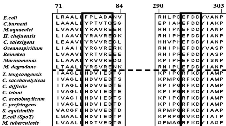
FIGURE 2. A charge reversal in a conserved motif distinguishes monofunctional and bifunctional Rel proteins. RXXD motif in bifunctional proteins is substituted by EXDD motif in monofunctional proteins (boxed). Bifunctional and monofunctional Rel proteins (separated by a dotted line) are grouped based on the presence or absence of HDXXED motifs (boxed). Relevant regions (containing these motifs) of the multiple sequence alignment of sequences representing these two groups are shown. The numbers above the alignment correspond to those of Rel Seq .
