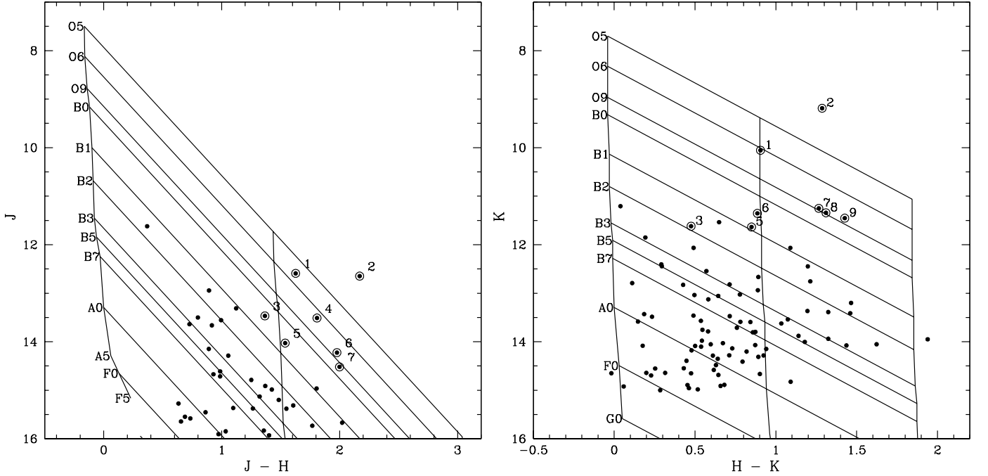
Fig. 3. Colour-magnitude diagrams of the infrared cluster in the IRAS 20178+4046 region. The nearly vertical solid lines represent the zero age main sequence (ZAMS) loci with 0, 15, and 30 magnitudes of visual extinction corrected for the distance. The slanting lines show the reddening vectors for each spectral type. The magnitudes and the ZAMS loci are all plotted in the Bessell & Brett (1988) system.
