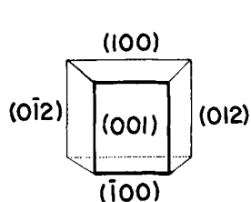
FIGURE 3 Schematic diagram of a single crystal of 2. The polar axis is along b . The faces (01\bar{2}) and (012) are present, the faces (0\bar{1}\bar{2}) and (0\bar{1}2) are not present.
