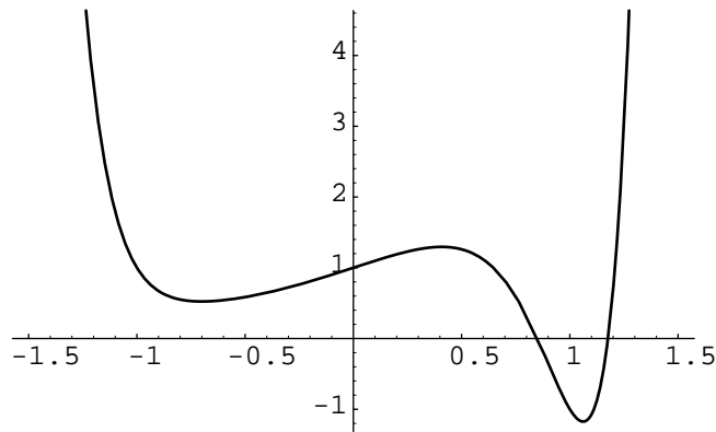
FIGURE 4.2. Real graph of the Lehmer polynomial
