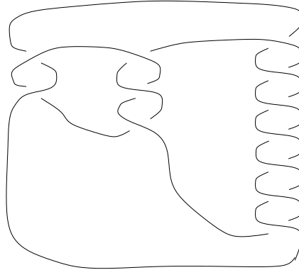
FIGURE 4.3. (-2,3,7) -pretzel knot
