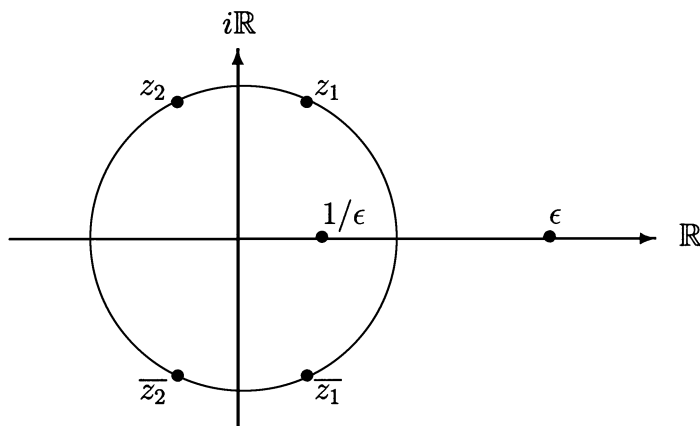
FIGURE 3.1. A (degree six) Salem number \epsilon and its conjugates
