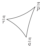
FIGURE 4.1. Fundamental domain of a (p, q, r) -hyperbolic triangle group
