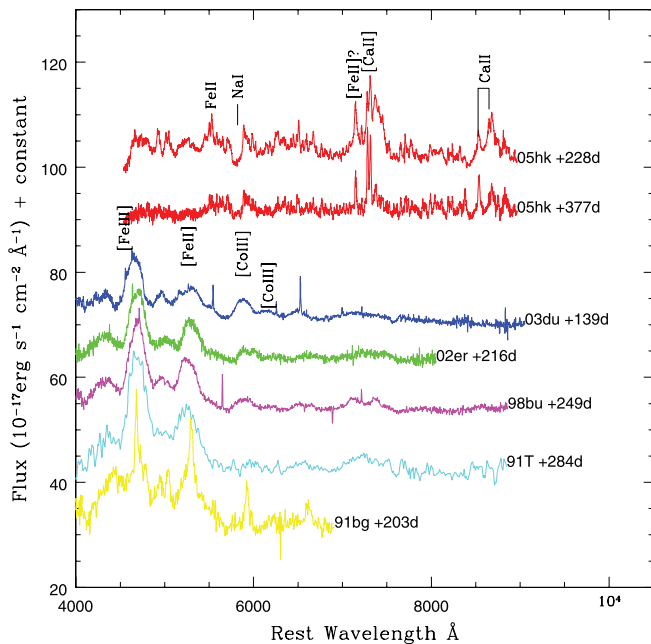
FIG. 14.—Same as Fig. 13, but compared with spectra of other Type Ia SNe: 2003du, 2002er, 1998bu, 1991T, and 1991bg.
