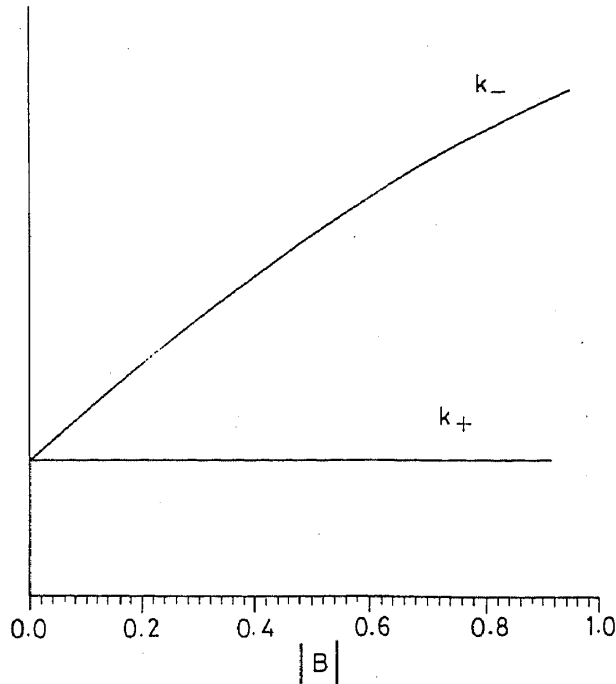
Figure 1. Plots of the fundamental modes k_{\pm} versus the coupling parameter |B| for a dielectric scatterer satisfying condition (8).
