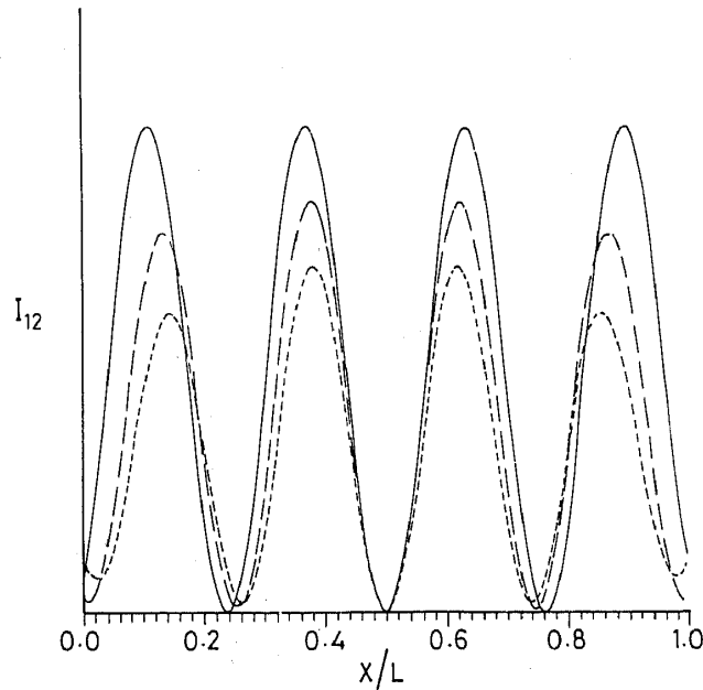
Figure 2. Plots of intensity I_{12} (in arbitrary units) versus relative position x/L at t=0 for a dielectric scatterer satisfying condition (8) with |B|=0 (—), |B|=1 (— — —), |B|=2 (- - - -).
