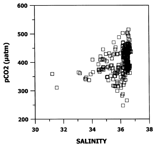
Figure 5. Relation between pCO 2 and salinity in the mixed layer in all seasons in the Arabian Sea.
