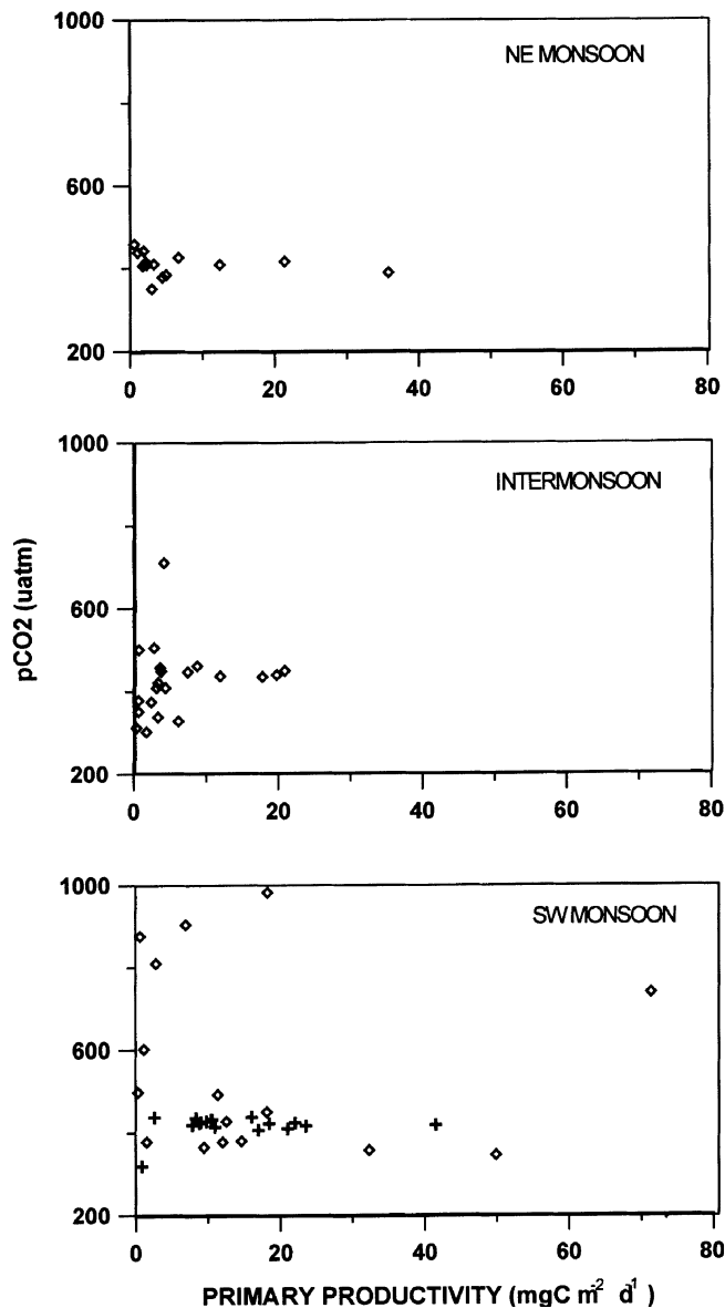
Figure 9. Relations for mixed layer p\text{CO}_2 with primary production in mixed layer during different seasons.
