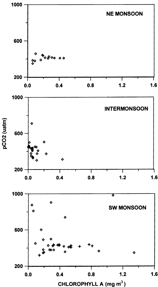
Figure 8. Relations for p\text{CO}_2 with chlorophyll a in mixed layer during different seasons.
