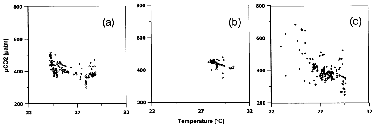
Figure 6. Relations for temperature with pCO_2 in the mixed layer in (a) NE- (b) inter and (c) southwest monsoon seasons.
