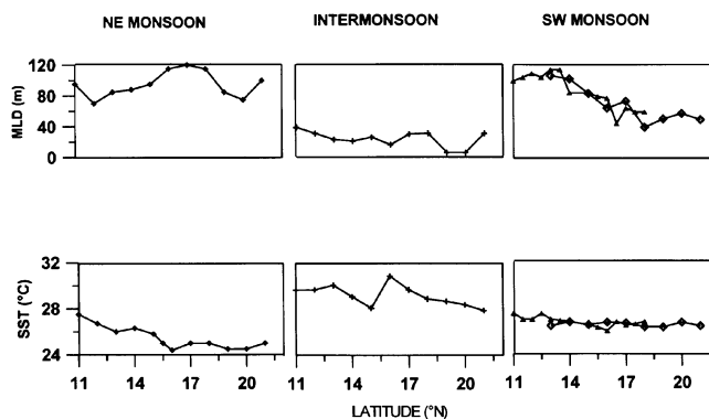
Figure 2. Seasonal variations in SST and MLD in the Arabian Sea along 64°E. In the right panel, triangles are for SW monsoon 1995 and diamonds for the same season of 1996.
