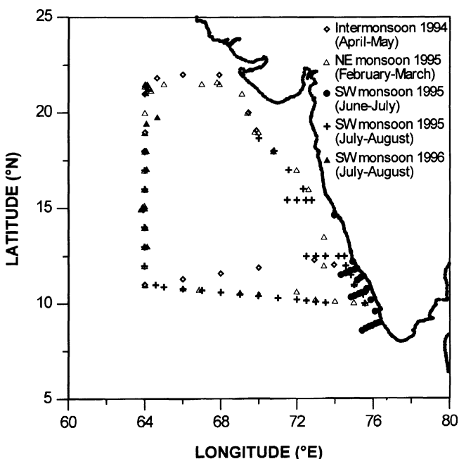
Figure 1. Station locations occupied in the JGOFS (India) cruises.
