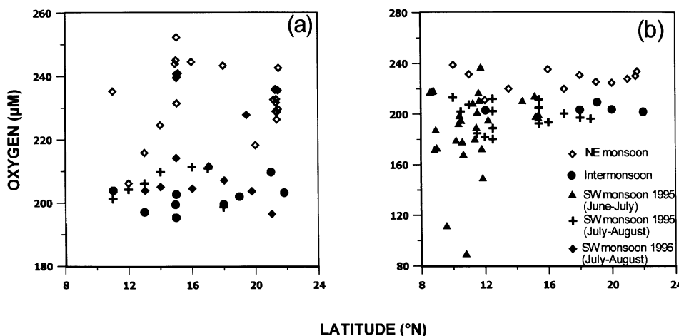
Figure 3. Variations in near surface dissolved oxygen (a) along 64°E and (b) along the west coast of India.
