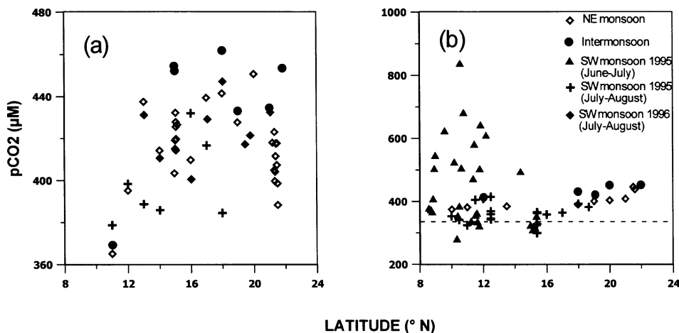
Figure 4. Variations in near surface pCO 2 (a) along 64E and (b) along the west coast of India. Dashed line in the right panel indicates atmospheric value.
