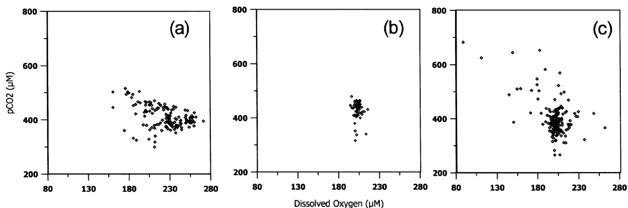
Figure 7. Relations for dissolved oxygen with pCO_2 in the mixed layers in (a) NE-, (b) inter and (c) southwest monsoon seasons.
