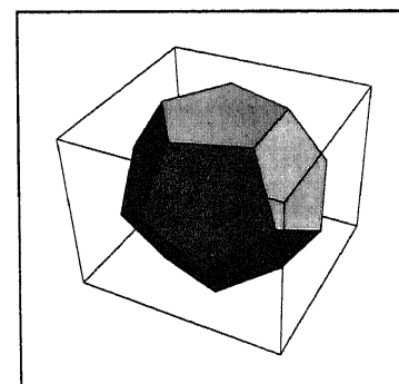
Figure 4 Dodecahedron.
