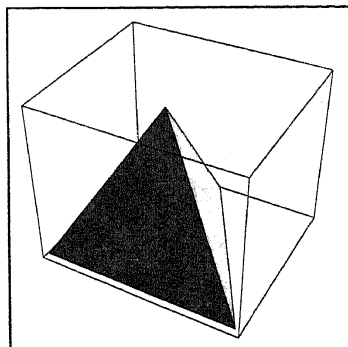
Figure 2 Tetrahedron.
