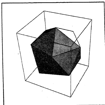
Figure 1 Icosahedron.
