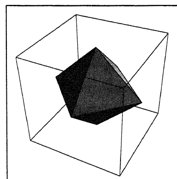
Figure 3 Octahedron.
