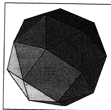
Figure 5 Snub cube.
