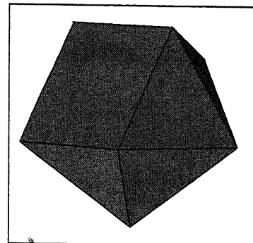
Figure 6 Square anti-prism.
