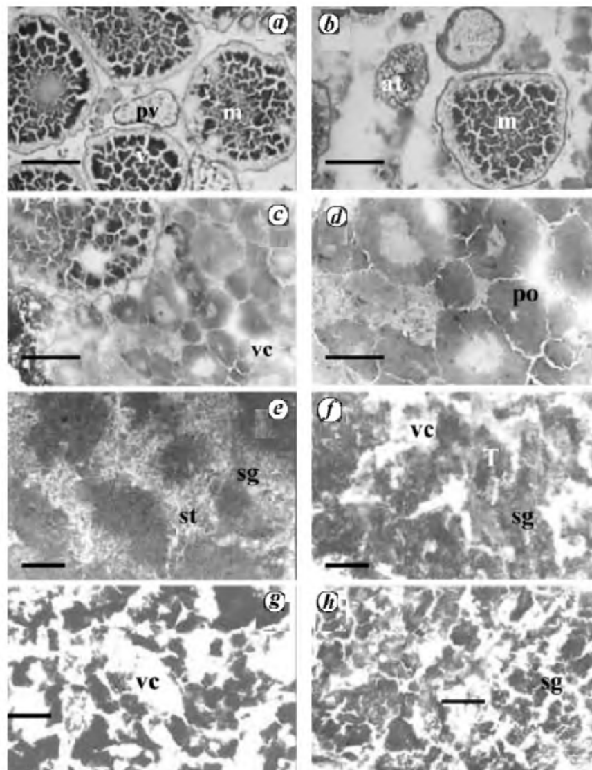
Figure 1. Effect of different doses of endosulfan on the gonad of zebrafish Danio rerio . a-d , Ovary: a , Control; b , 350 ng/l; c , 1050 ng/l and d , 1400 ng/l. at, Atretic oocyte; m, Matured oocyte; po, Primary oocyte; pv, Pre-vitellogenic oocyte; v, Vitellogenic oocyte; vc, Vacuole. Scale: 300 \mu m. e-h , Testis: e , Control; f , 44 ng/l; g , 700 ng/l and h , 1050 ng/l. sg, Spermatogonium; st, Spermatids; T, Seminiferous tubule and vc, Vacuole. Scale: 25 \mu m.
