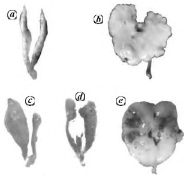
Figure 2. Matured testis (a) and ovary (b) representative partially differentiated testis (c and d) and ovary (e) of juvenile gonads of the zebrafish, which were previously treated with endosulfan.
