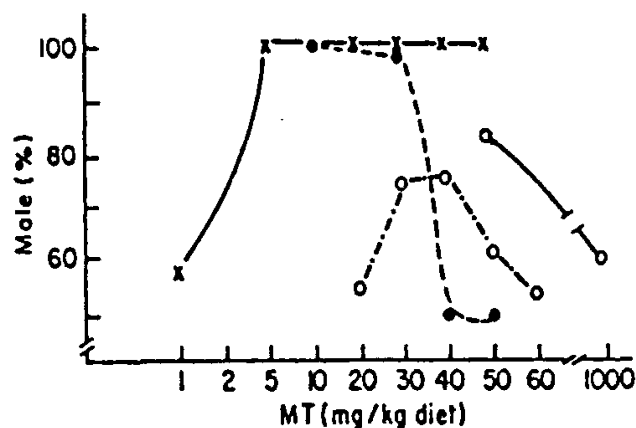
Figure 1. Variations in the sex-reversing potency of 17 \alpha -methyltestosterone administered through diet by different authors: o---o, Clemens and Inslee; o----o, Nakamura; o—o, Das et al. ; x—x, Pandian and Varadaraj (all from Pandian and Varadaraj 15 ).
