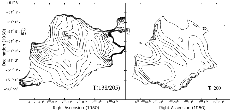
Figure 8. The distribution of dust temperature T(138/205) , and optical depth at 200\mu\text{m} , \tau_{200} , for the region around S209 assuming a dust emissivity law of \epsilon_\lambda \propto \lambda^{-2} . The isotherms refer to the same temperatures as in Fig. 7. The \tau_{200} contours represent 100, 75, 50, 25 & 12.5 % of the peak value of 0.67.
