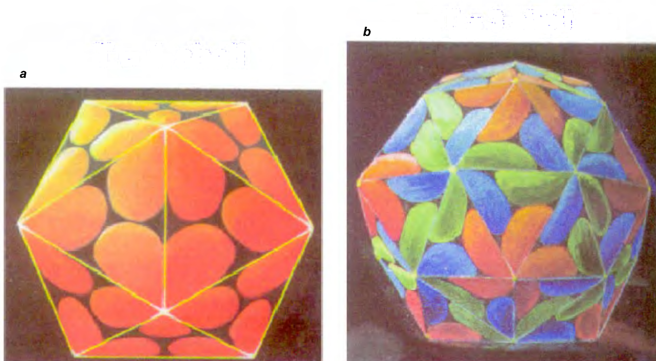
Figure 1. Arrangement of subunits in (a) T=1 and (b) T=3 icosahedral capsids of isometric viruses. All subunits of T=1 capsids are in chemically identical environments. Subunits on T=3 capsids, although identical in sequence, occur in three distinct environments. These subunits are designated A (red), B (blue) and C (green) following Harrison et al. 20 . The A (red) subunits form pentamers at the icosahedral five-fold axes, while B and C subunits form hexamers at the icosahedral three-fold axes.
