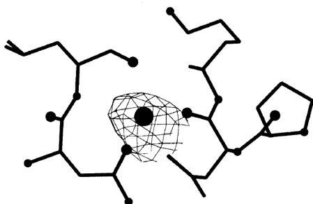
Figure 4. Difference Fourier section, contoured at 2.5 \sigma , showing the electron density for a bound ion. The ion was identified as a calcium ion by comparison with the T3-SeMV structure.
