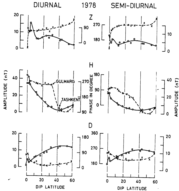
Figure 3. Latitudinal variations of the amplitude (solid line) and phase (broken line) of the diurnal and semi-diurnal terms of daily variations in the three geomagnetic components D, H and Z.
