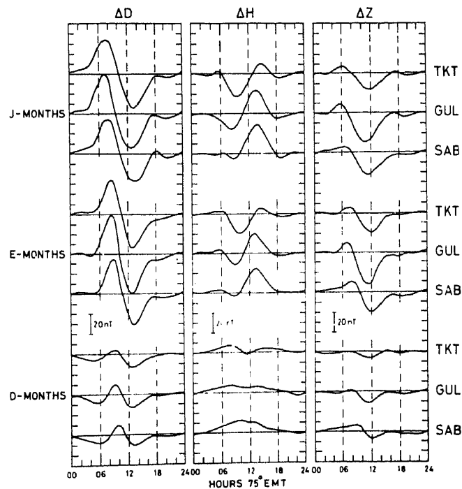
Figure 4. Mean seasonal quiet-day variations in D, H and Z at Sabhawala, Gulmarg and Tashkent for the year 1978.
