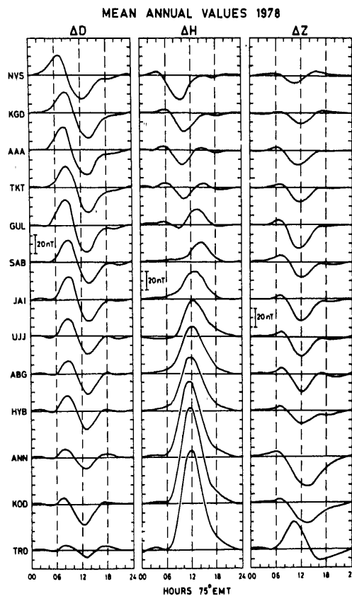
Figure 2. Solar quiet-day variations in geomagnetic field components, D, H and Z at magnetic observatories along Indian longitudinal belt for the year 1978.
