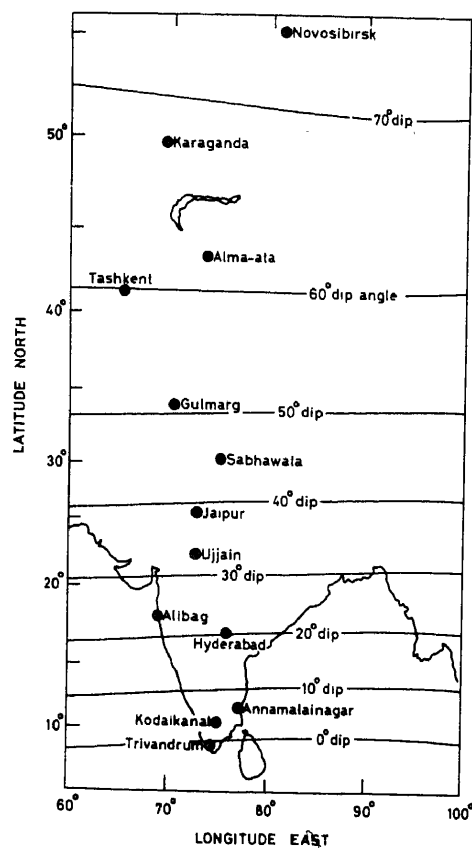
Figure 1. Map showing the locations of magnetic observatories whose data are used in the present analysis.
