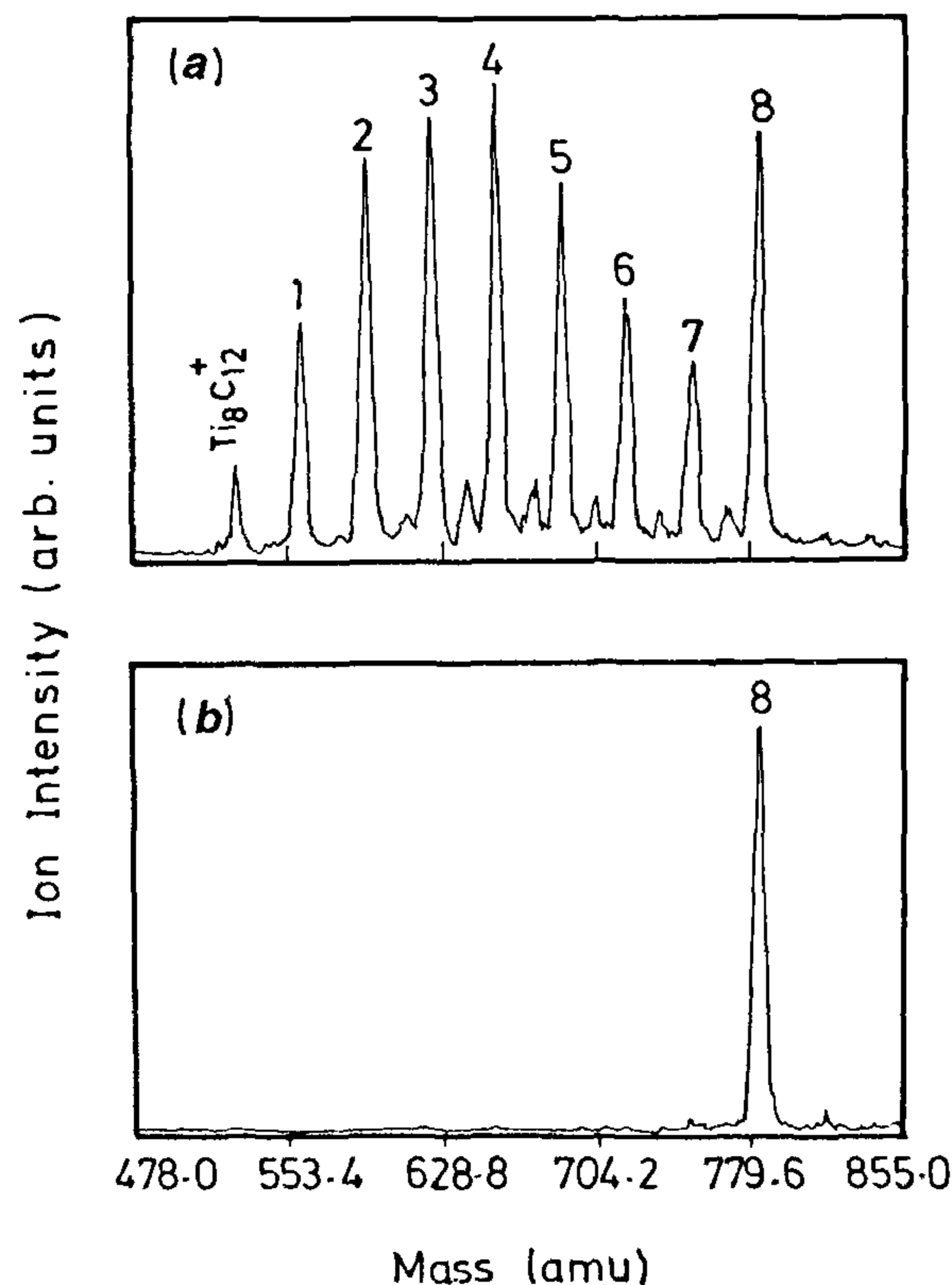
Figure 8. Mass spectra of the reaction products of methanol with Ti_8C_{12}^+ . a , low partial pressure of methanol, b , much higher partial pressure of methanol (From ref 16, used with permission)
