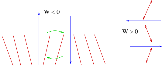
FIG. 7: The heart of the generic instability of ordered active filaments: long-wavelength splay produces shear flows that further distort a row of parallel contractile force dipoles (left); similarly bend disrupts extensile filaments (right).
