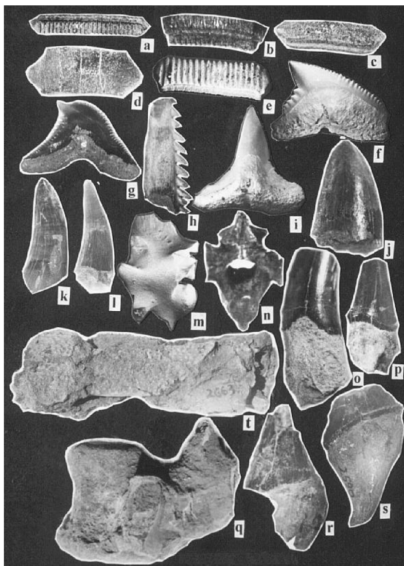
Figure 2. Vertebrates from Panandhro lignite mine. a, (× 4); b, (× 3); c, (× 3); d, (× 3.5); e, (× 4); h, (× 1.5) Myliobatis sp. isolated teeth and spine (RUSB 301305, 306); f, (× 3) Galeocerdo isolated tooth (RUSB 307); g, (× 3) Selachii indet. isolated tooth (RUSB 308); i, (× 4.5) Isurus sp. isolated tooth (RUSB 309); j, (× 3); k, (× 3); l, (× 3); q, (× 0.75) Crocodylidae indet. isolated teeth and vertebra (RUSB 310313); m, (× 5); n, (× 3.5) Serpentes indet. vertebrae (RUSB 314, 315); o, (× 2); p, (× 3); r, (× 3); s, (× 2) Kutchicetus minimus ? isolated mammal teeth (RUSB 2579, 2589, 2578, 2590); t, (× 0.75) Arius kutchensis fragmentary skull (RUSB 316).
