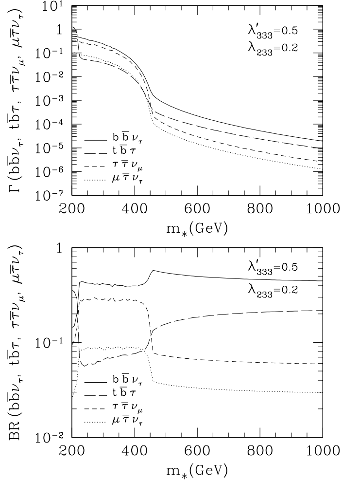
Figure 12: Widths (in GeV) and branching ratios for the four decays \tilde{\chi}_1^0 \rightarrow b\bar{b}\nu_\tau , t\bar{b}\tau , \tau\bar{\tau}\nu_\mu , and \mu\bar{\tau}\nu_\tau , when only the two couplings \lambda'_{333} and \lambda_{233} are nonvanishing, as function of the sfermion mass m_* , equal to m_{\tilde{Q}} = m_{\tilde{U}^c} = m_{\tilde{D}^c} , and m_{\tilde{L}} = m_{\tilde{E}^c} , for \mu = 500 GeV, m_{\tilde{B}} = 500 GeV, and m_{\tilde{W}} = 2m_{\tilde{B}} . The value of \tan\beta is 3 and all trilinear soft terms are chosen in such a way to have vanishing left-right mixing terms in the sfermion mass matrices squared.
