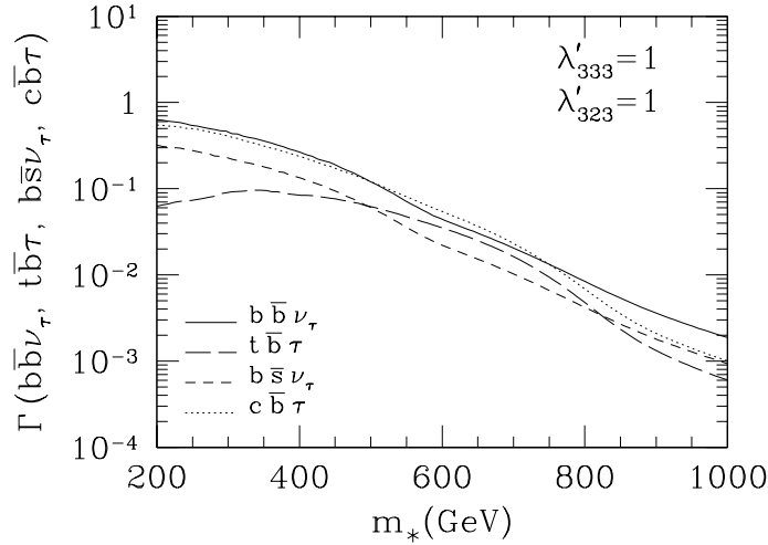
Figure 11: Widths (in GeV) for the four decays \tilde{\chi}_1^0 \rightarrow b\bar{b}\nu_\tau , t\bar{b}\tau , b\bar{s}\nu_\tau , and c\bar{b}\tau , when only the two couplings \lambda'_{333} and \lambda'_{323} are nonvanishing, as function of the sfermion mass m_* , equal to m_{\tilde{Q}} = m_{\tilde{U}^c} = m_{\tilde{D}^c} , and to (1.4) \times m_{\tilde{L}} (with m_{\tilde{L}} = m_{\tilde{E}^c} ), for \mu = 1500 GeV, m_{\tilde{B}} = 600 GeV, and m_{\tilde{W}} = 2m_{\tilde{B}} . The value of \tan\beta is 3 and all trilinear soft terms are chosen in such a way to have vanishing left-right mixing terms in the sfermion mass matrices squared.
