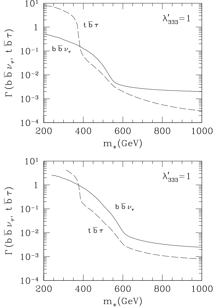
Figure 9: \Gamma(\tilde{\chi}_1^0 \rightarrow b\bar{b}\nu_\tau) and \Gamma(\tilde{\chi}_1^0 \rightarrow t\bar{b}\tau) (in GeV), respectively solid and long-dashed lines, versus m_* = m_{\tilde{Q}} = m_{\tilde{U}^c} = m_{\tilde{D}^c} , for \mu = 600 GeV, m_{\tilde{L}} = m_{\tilde{E}^c} = 600 GeV, m_{\tilde{B}} = 600 GeV, and m_{\tilde{W}} = 2m_{\tilde{B}} . The value of \tan\beta is 3 in the upper frame, 30 in the lower one. All trilinear soft terms are fixed at 350 GeV in the upper frame, and at 150 GeV in the lower frame.
