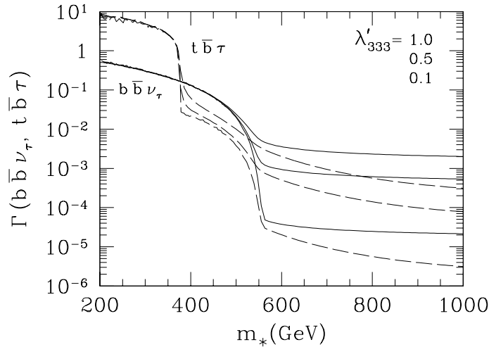
Figure 10: Dependence of \Gamma(\tilde{\chi}_1^0 \rightarrow b\bar{b}\nu_\tau) (solid lines) and \Gamma(\tilde{\chi}_1^0 \rightarrow t\bar{b}\tau) (long-dashed lines) on the coupling \lambda'_{333} . All other parameters are chosen as in the upper frame of figure 9. The values of \lambda'_{333} are 1, 0.5, 0.1 from top to bottom.
