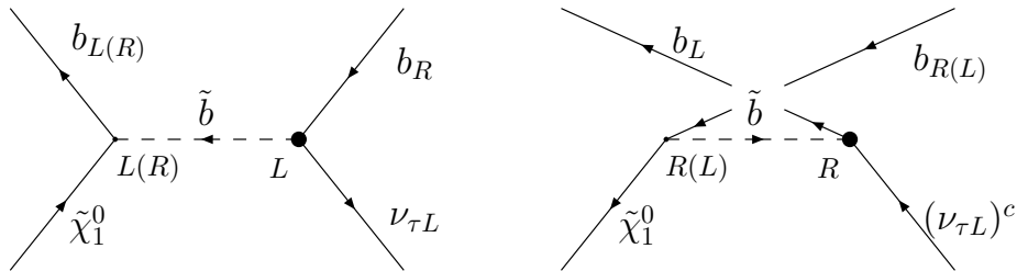
Figure 1: Diagrams contributing to the decay \tilde{\chi}_1^0 \rightarrow b\bar{b}\nu_\tau through the exchange of a virtual \tilde{b} -squark. The thick vertex indicates the R_p -violating coupling \lambda_{333}^* . The labels L and R at each vertex indicate the chirality of the ingoing and/or outgoing scalar fields. To the same decay contribute also the crossed diagrams, i.e. those with the two external bottom-quarks interchanged and an ingoing neutrino line, and with the thick vertex indicating the R_p -violating coupling \lambda'_{333} .
