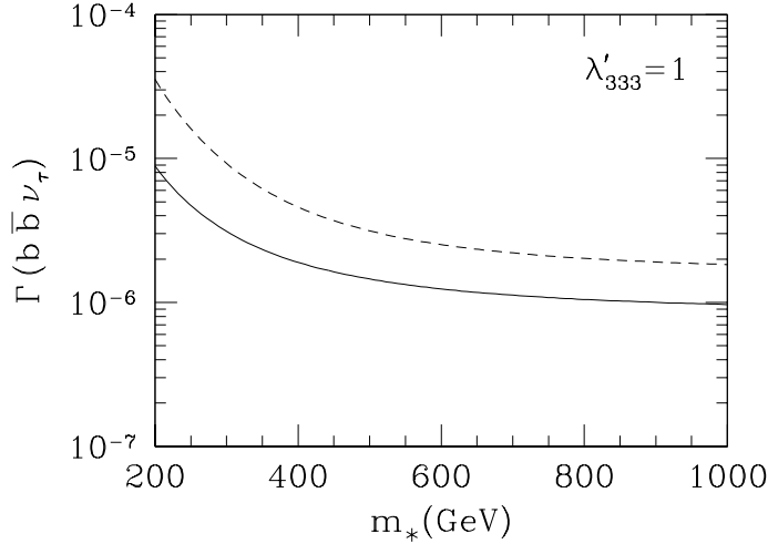
Figure 7: \Gamma(\tilde{\chi}_1^0 \rightarrow b\bar{b}\nu_\tau) (in GeV) versus m_* = m_{\tilde{Q}} = m_{\tilde{U}^c} = m_{\tilde{D}^c} for the decay of an almost pure gaugino \tilde{\chi}_1^0 for \mu = 500 GeV, \tan\beta = 3 , m_{\tilde{L}} = m_{\tilde{E}^c} = 400 GeV, and gaugino masses m_{\tilde{B}} = (1/2)m_{\tilde{W}} = 100 GeV (solid lines), m_{\tilde{W}} = (1/2)m_{\tilde{B}} = 100 GeV (dashed lines). The trilinear soft terms were chosen in such a way to cancel the left-right mixing terms in all sfermion mass matrices.
