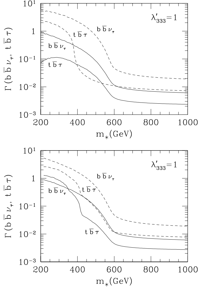
Figure 8: \Gamma(\tilde{\chi}_1^0 \rightarrow b\bar{b}\nu_\tau) and \Gamma(\tilde{\chi}_1^0 \rightarrow t\bar{b}\tau) (in GeV) versus m_* = m_{\tilde{Q}} = m_{\tilde{U}^c} = m_{\tilde{D}^c} , for \mu = 1500 GeV, \tan\beta = 3 , m_{\tilde{L}} = m_{\tilde{E}^c} = 600 GeV. The gaugino masses are m_{\tilde{B}} = (1/2)m_{\tilde{W}} = 600 GeV (solid lines), m_{\tilde{W}} = (1/2)m_{\tilde{B}} = 600 GeV (dashed lines). The trilinear soft terms are chosen in such a way to give vanishing left-right entries in all sfermion mass matrices in the upper frame and moderate left-right entries the lower frame.
