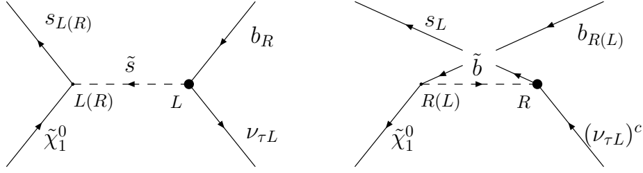
Figure 5: Diagrams contributing to the decay \tilde{\chi}_1^0 \rightarrow s\bar{b}\nu_\tau through the exchange of a virtual \tilde{s} - and \tilde{b} -squark. The thick vertex indicates the R_p -violating coupling \lambda_{323}^{*} .
