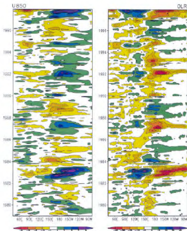
Figure 3. Time-longitude section of mean monthly external anomalies of zonal winds at 850 hPa ( m^2 s^{-2} ) and OLR ( Wm^{-2} ) 2 averaged around equator (5°S-5°N).
