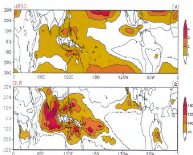
Figure 10. Internal variance of (a) zonal winds at 850 hPa ( \text{m}^2 \text{s}^{-2} ) and (b) OLR ( \text{Wm}^{-2} ) 2 based on all months after removing the higher frequencies with period shorter than 10 days.
