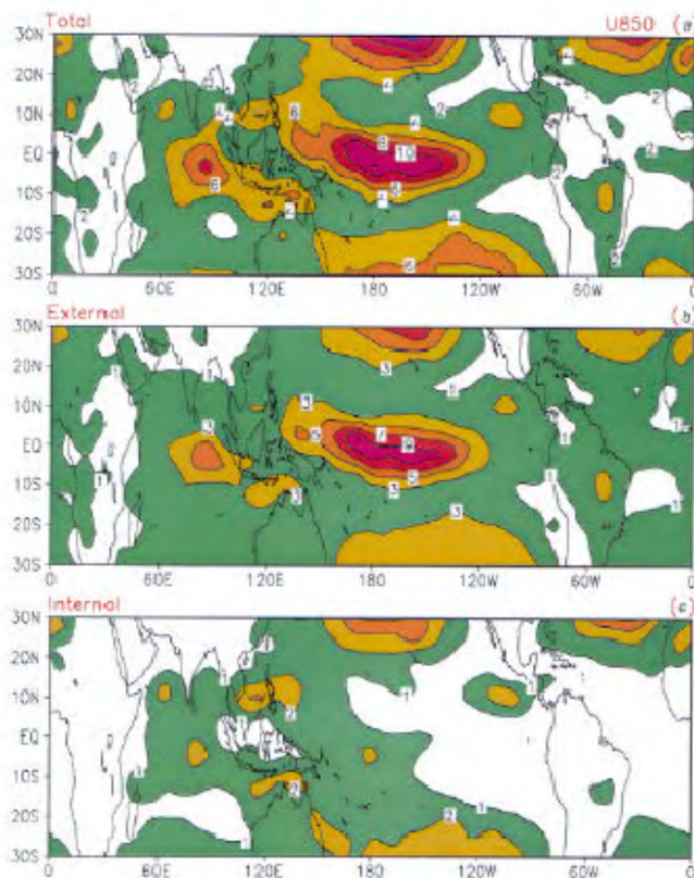
Figure 4. Monthly variance of zonal winds ( \text{m}^2 \text{s}^{-2} ) at 850 hPa based on 396 months for the period January 1956 to December 1997. a , Total variance; b , external variance; and c , internal variance.
