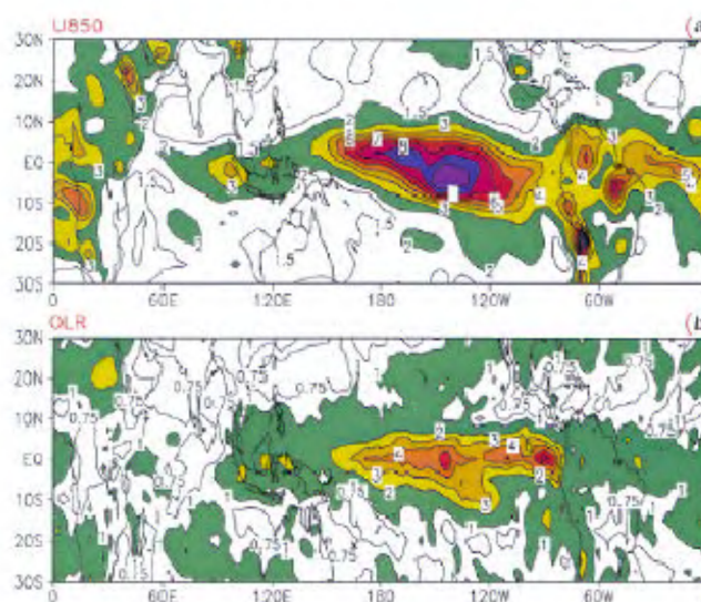
Figure 6. Predictability index for (a) zonal winds at 850 hPa (396 months); and (b) OLR (288 months).
