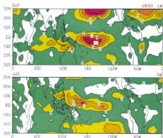
Figure 8. External variance of zonal winds at 850 hPa ( \text{m}^2 \text{s}^{-2} ) during ( a ) NH winter months (December–February); and ( b ) during NH summer months (June–August).
