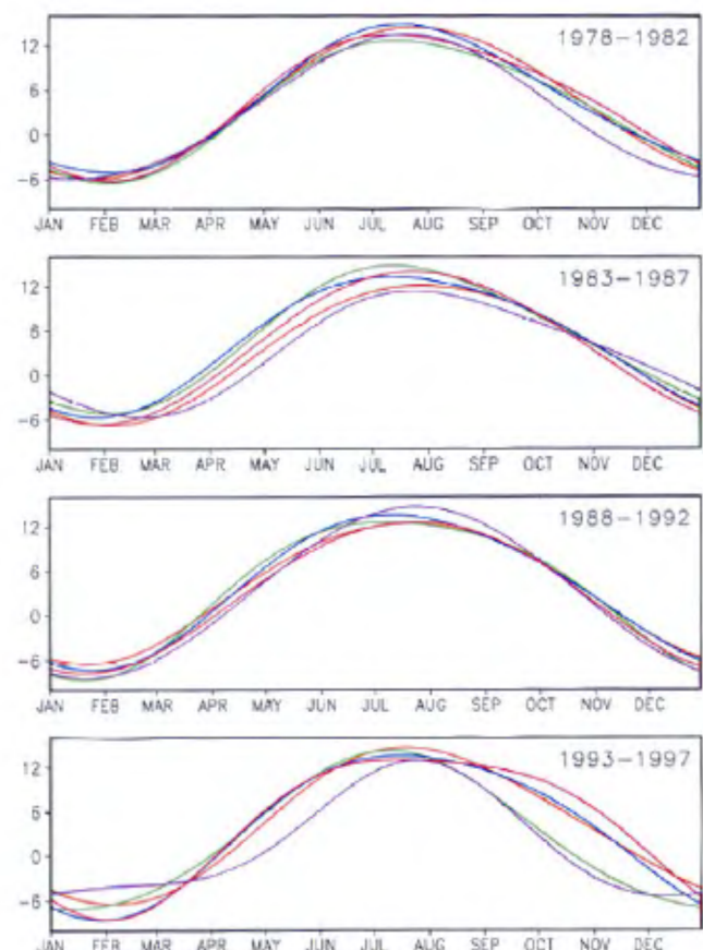
Figure 1. Illustration of variations of the annual cycle from year to year. The annual cycles of zonal winds ( \text{ms}^{-1} ) at 850 hPa at a point ( 80^{\circ}\text{E} , 5^{\circ}\text{N} ) are shown for 20 years.
