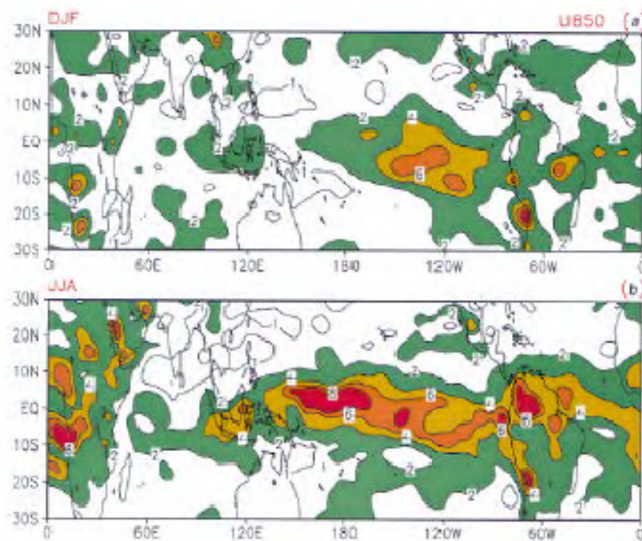
Figure 7. Predictability index for zonal winds at 850 hPa ( a ) for all northern hemisphere winter months (December–February); and ( b ) for all northern hemisphere summer months (June–August).
