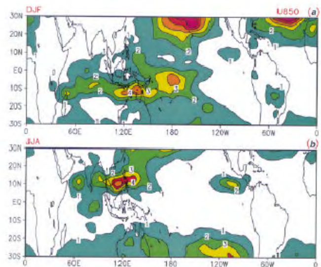
Figure 9. Internal variance of zonal winds at 850 hPa ( \text{m}^2 \text{s}^{-2} ) during ( a ) NH winter months (December–February); and ( b ) during NH summer months (June–August).
