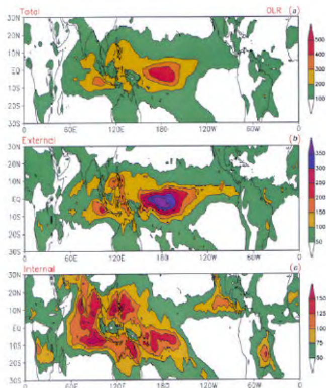
Figure 5. Same as Figure 4, but for OLR for the period January 1974 to December 1997 (288 months). Units ( \text{Wm}^{-2} ) 2 .
